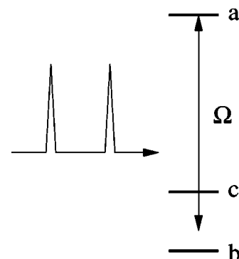
FIG. 1. Schematic of atomic levels.
