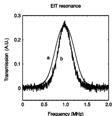
FIG. 4. Transmission of laser radiation vs frequency of repetition rate ( 1/T ) for short pulses. The repetition rate changes around 506 MHz, which is one-sixth of the hf splitting (sixth subharmonic).
