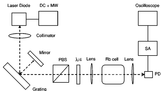
FIG. 2. Schematic of the experimental setup. PBS, polarizing beam splitter.
