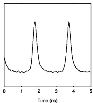
FIG. 3. Optical pulses generated by the mode-locked diode laser. Period between pulses T is about 2 ns which is six times larger than the period of oscillation of the coherence between sublevels of the ground state.
