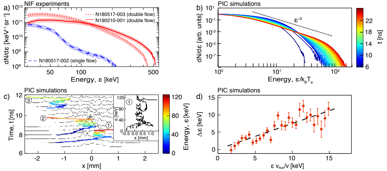
Figure 4: Non-thermal electron acceleration. a) Comparison of the measured time-integrated electron spectrum in double flow (solid and dotted red) and single flow (dashed blue) experiments indicates that when a shock is formed electrons are accelerated up to 500 keV. Shaded regions indicate error bars of \pm 25\% corresponding to a systematic error in the image plate response of the electron spectrometer. b) Evolution of the electron spectrum (colored by time) in the shocked region obtained in simulations confirms that the shock accelerates electrons to \gtrsim 100k_B T_e , leading to the formation of a non-thermal power-law tail \epsilon^{-p} with a spectral index p = 3 (dotted). c) Trajectories of three representative non-thermal electrons (colored by energy) overlaid on the magnetic energy profile (black lines) show energization due to stochastic interactions with the turbulent fields within the shock transition. The inset shows that electrons can gain energy via multiple reflections along the flow axis ( x ) as they are trapped in the shock transition layer. d) The average energy gain experienced by electrons in each reflection (red dots) is consistent with a first-order Fermi process (dashed curve shows linear fit). Error bars indicate the standard error of the mean.
