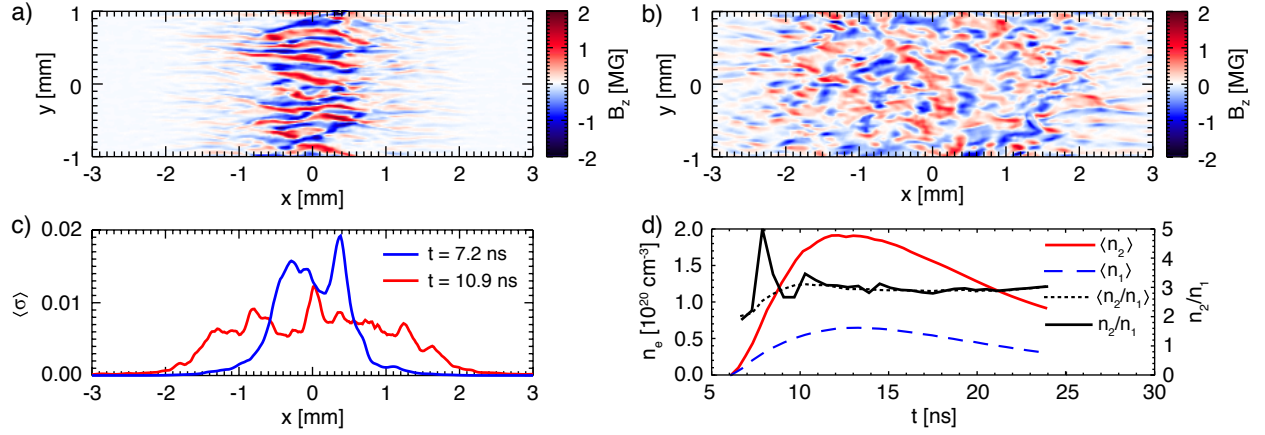
Figure 3: 2D particle-in-cell simulation of the shock structure. Magnetic field maps are shown at a) 7.2 ns and b) 10.9 ns, indicating the generation of turbulent MG fields associated with the Weibel instability. c) The spatially averaged ratio of magnetic energy density to flow energy density ( \sigma ) reaches > 1\% in the shocked (downstream) plasma. d) Evolution of the spatially averaged single flow ( n_1 , dashed blue) and double flow ( n_2 , solid red) density at the center of the interaction region. The shock is formed at 9 ns when the compression ratio (dotted black) between downstream ( n_2 ) and upstream ( n_1 ) densities reaches n_2/n_1 \sim 3 , as predicted from the 2D shock jump conditions (instead of n_2/n_1 \sim 4 in 3D). The compression ratio measured in the simulation for a small region corresponding to the Thomson scattering probing volume (solid black) shows large modulations during the shock formation phase ( \lesssim 9 ns), associated with the development of small-scale turbulence. Note that the simulation uses a periodic box transversely and thus cannot capture the transverse expansion of the plasma after shock formation and subsequent decay in density.
