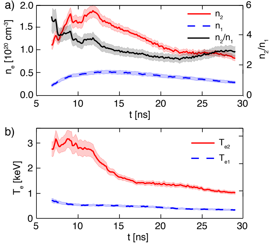
Figure 2: Thomson scattering measurements indicating shock formation. a) Evolution of the electron density at the central region of the experiment for single flow ( n_1 , dashed blue) and two colliding flows ( n_2 , solid red). The compression ratio (black) between downstream ( n_2 ) and upstream ( n_1 ) densities reaches n_2/n_1 \gtrsim 4 at early times ( < 10 ns) indicating shock formation. b) Evolution of the electron temperature for single flow ( T_{e1} , dashed blue) and colliding flows ( T_{e2} , solid red) shows significant heating of the shocked (downstream) electrons to 3 keV. As the shocked plasma expands in the transverse direction (see Figure 1a), the compression ratio and plasma temperature slowly decrease in time. The error in the measurements is indicated by the shaded regions and corresponds to the standard deviation of the fit of the Thomson scattering spectrum to the plasma parameters.
