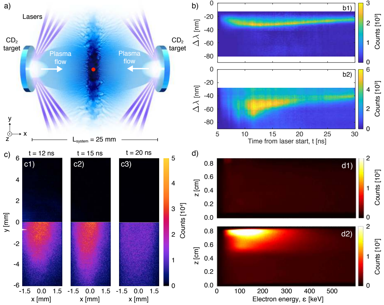
Figure 1: Laser-driven collisionless shock experiments. a) Sketch of the experimental setup with shock density structure (in blue) obtained from numerical simulation. b) Thomson scattering data provides measurement of electron density and temperature at the central region (marked by red dot in a) for a b1) single flow and b2) two colliding flows. c) Comparison of the X-ray self-emission from the plasma between a single flow (top) and colliding flows (bottom) indicates strong compression and heating of the shocked plasma. d) Spectrometer measurements of fast electrons ( > 30 \text{ keV} ) produced in d1) a single flow and d2) two colliding flows demonstrate acceleration of electrons to relativistic energies.
