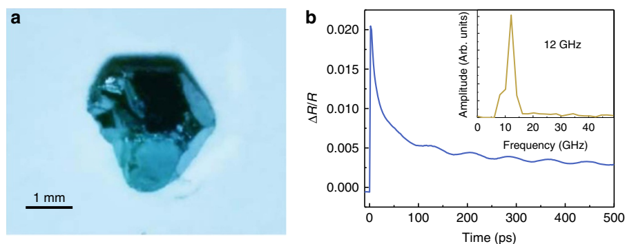
Figure 2 | Transient reflectivity of \text{CH}_3\text{NH}_3\text{PbI}_3 single crystal. (a) Photograph of the \text{CH}_3\text{NH}_3\text{PbI}_3 single crystal annealed at 100 °C. (b) Transient reflectivity signal obtained on the sample annealed at 100 °C at a pump wavelength of 550 nm and a probe wavelength of 850 nm. Inset: Fourier transform of the electronic background subtracted transient reflectivity.
