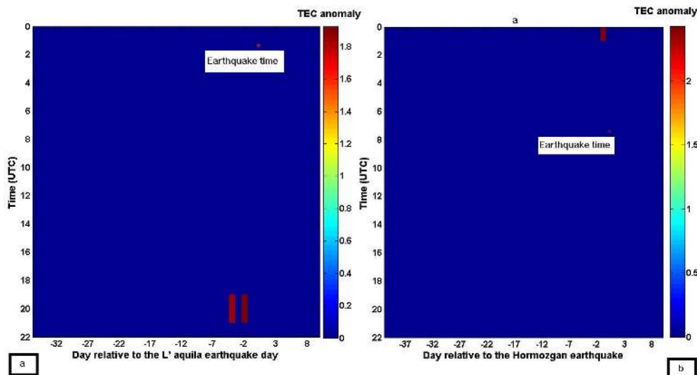
Fig. 5. Results of TEC anomaly analysis. (a) Detected TEC anomalies for the L'Aquila earthquake (6 April 2009) from 1 March to 16 April 2009 based on |D\text{TEC}| > 1.5 , K_p < 2.5 and D_{st} > -20 (nt). The y-axis represents the time UTC (LT=UTC+02:00). (b) Detected TEC anomalies for the Hormozgan earthquake (28 February 2006) from 18 January to 8 March 2006 based on |D\text{TEC}| > 2.0 , K_p < 2.5 and D_{st} > -20 (nt). The y-axis represents the time UTC (LT=UTC+03:30).
