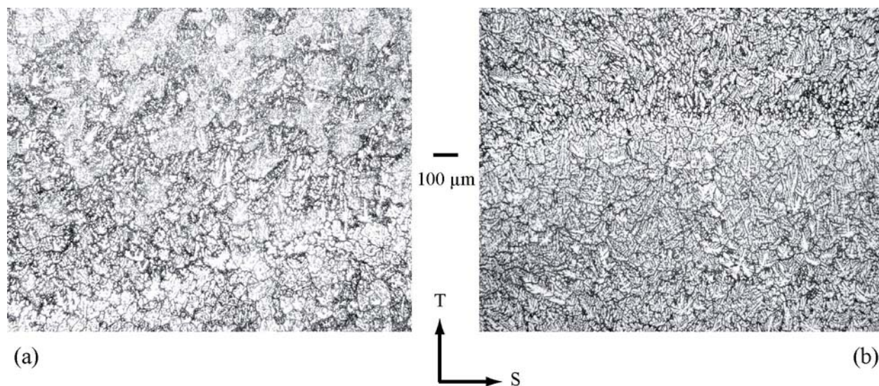
Figure 2. Microstructures of EBF 3 2219 Al deposits showing range of microstructures achievable: (a) low translation speed results in inhomogeneous microstructure and larger grains, and (b) higher translation speed produces more homogeneous microstructure with smaller equiaxed grains. [7]
