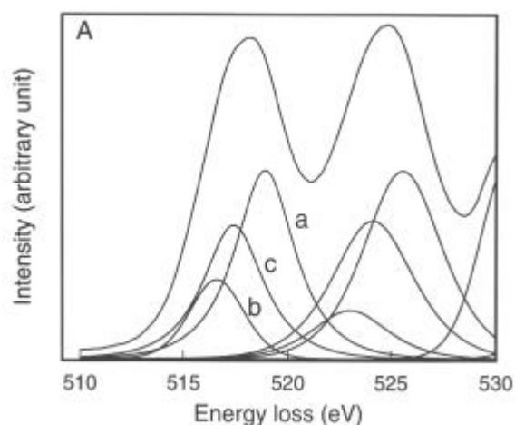
Figure 5A: V 2p ELNES after 7 min irradiation. The V 2p_{3/2} peak can be fitted as a sum of two Gauss curves a for V_2O_5 (max. at 519 eV) and b for VO (max. at 516.5 eV) resulting in c (max. at 517.5 eV) for the intermediate phase.
