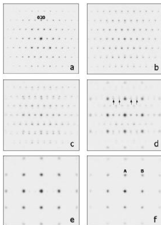
Figure 2: Electron diffraction patterns at irradiation times during which the corresponding energy loss spectra of Fig. 1 were recorded. The spots marked by arrows disappear for prolonged irradiation.
