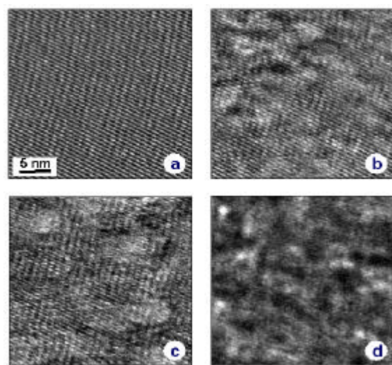
Figure 3: High-resolution images of V_2O_5 during irradiation. Irradiation times: a: 0 min; b: 7 min; c: 10 min; d: 15 min. The V_2O_5 specimen is oriented slightly off the 001 axis.
