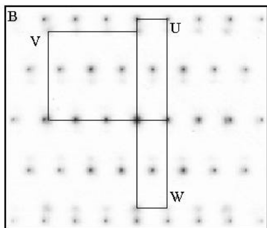
Figure 5B: electron diffraction pattern after 7 min irradiation. The reciprocal unit cells of the V_2O_5 , VO, and the intermediate phase are indicated by U, V, W, respectively.
