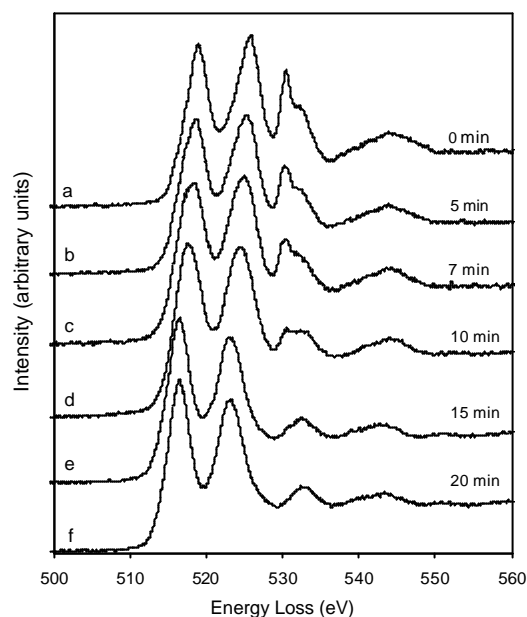
Figure 1: V 2p and O 1s ELNES of V 2 O 5 as a function of irradiation time. Spectra are offset for distinction. The electron current density was 3 A/cm 2 .
