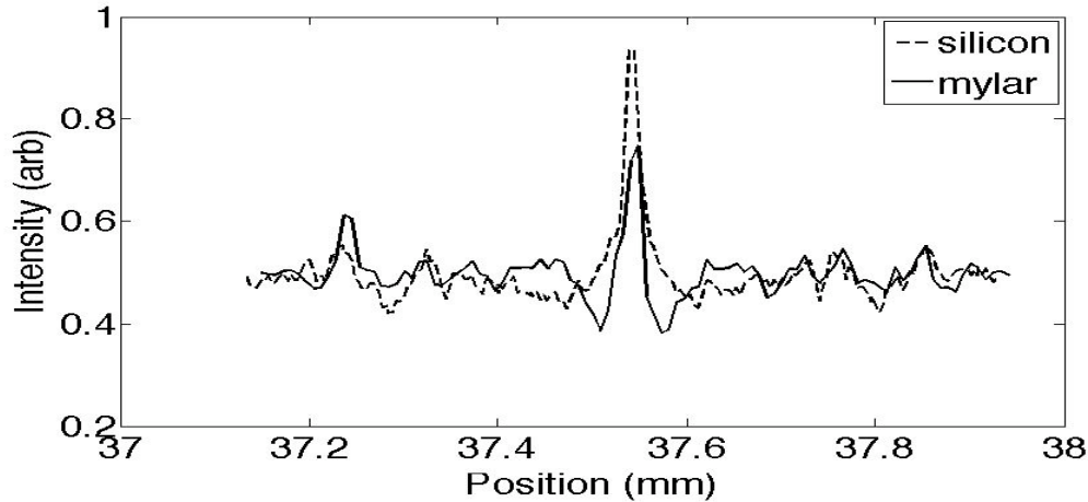
FIGURE 3. The silicon trace has clearly improved over the mylar one. The dips are no longer present, and wings on either side of the main peak, which are indicative of a head or tail on the bunch can now be seen. Structures are visible at large delay on both traces, indicating either poor response of the detector and/or absorption in air that must still be resolved.
