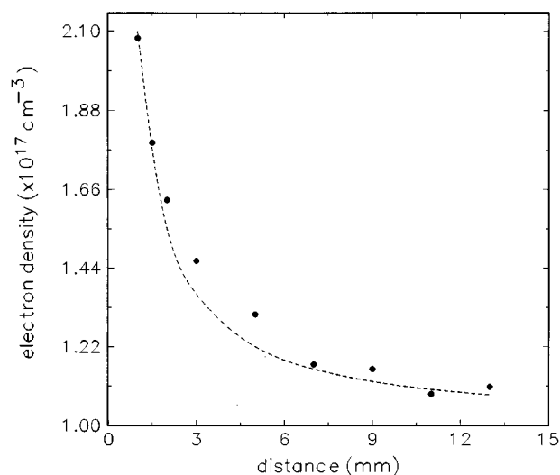
FIG. 3. Electron density of the graphite plasma as a function of distance from the target surface. The dotted line represents 1/z curve (laser irradiance used 50 \text{ GW cm}^{-2} ).
