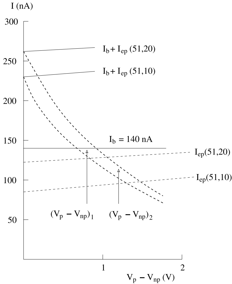
Figure A2. I_{\text{php}} as a function of (V_p - V_{\text{np}}) in 2006. For I_b = 140 nA and I_e \ll I_b , (V_p - V_{\text{np}})_1 = (0.9 \pm 0.2) V. See text for discussion about (V_p - V_{\text{np}})_2 .
