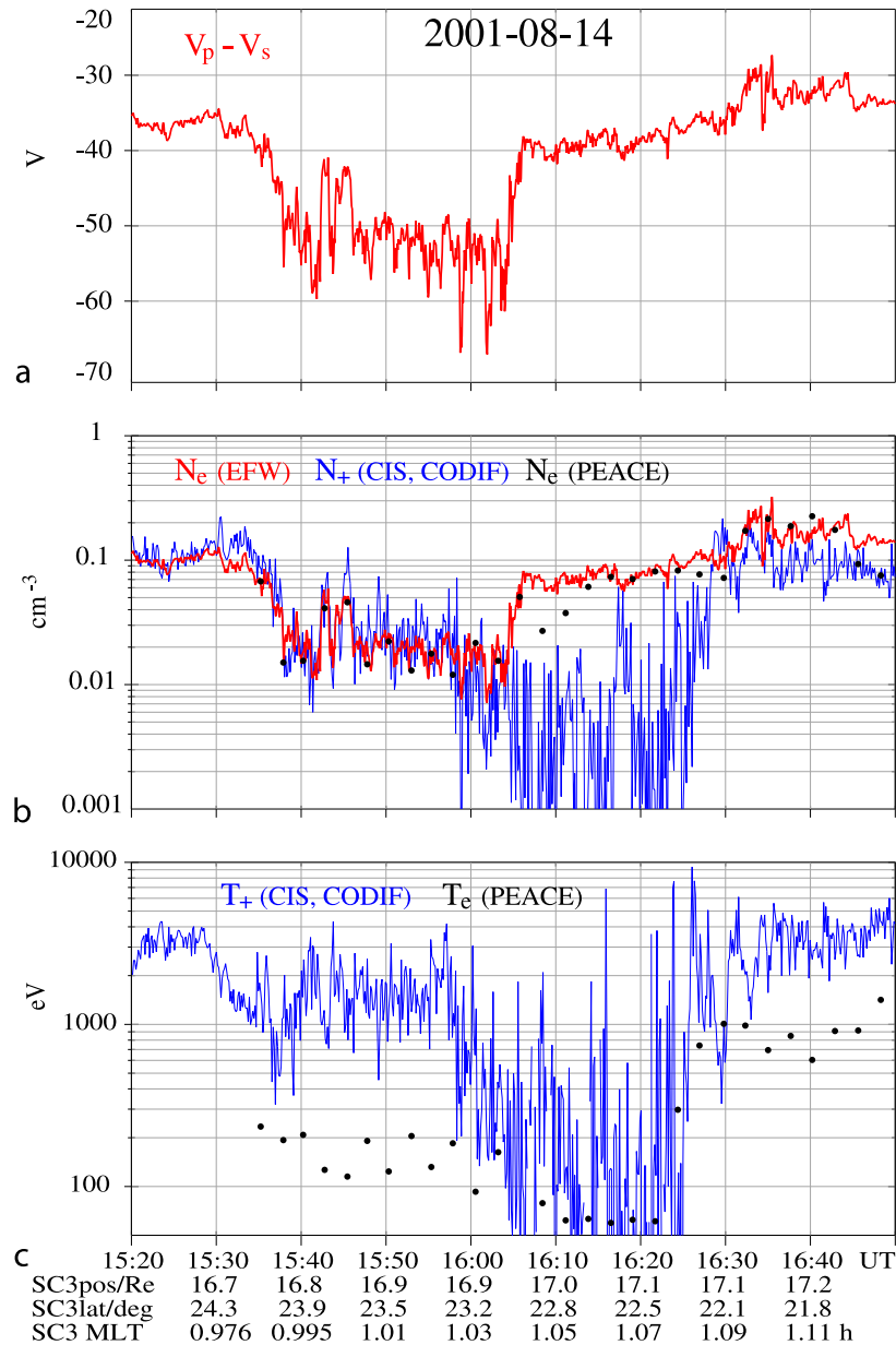
Figure 14. Measurements in the plasma sheet and plasma sheet boundary layer. (a) The probe-spacecraft potential difference ( V_p - V_s ); (b) N_c (EFW), N_+ (CIS) and N_c (PEACE) from moment calculations presented as black dots; (c) T_+ (CIS) from prime parameters and T_c (PEACE) from moment calculations.
