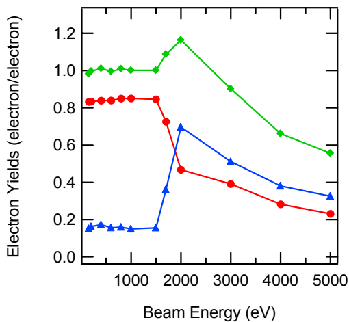
FIG. 4. DC-total ( \blacklozenge ), SE ( \bullet ), and BSE ( \blacktriangle ) yields for Al2219. The sample remained charged until 1500 eV, where dielectric breakdown occurred.
