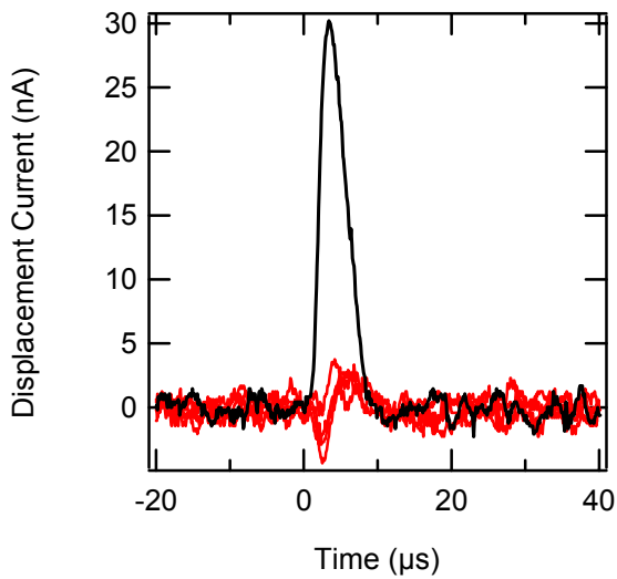
FIG. 15. Shown is a plot of the rise in displacement current of a probing electron pulse (5 \mu s at 100 nA) once the incident energy overcame the surface potential barrier induced by a high-energy electron beam. In this case, the small displacement currents are induced by probe beam energies ranging from 900-1200 eV, while the large displacement current curve occurred at 1250 eV. From this, the surface potential was taken to be 1250 eV.
