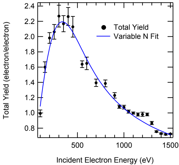
FIG. 12. Pulsed-yield curve versus beam energy for DC 93-500 sample 6 with flood gun neutralization after each pulse. Each yield point was the average of 50 pulsed-yield measurements ( 5 \mu\text{s} pulse with amplitude 50 nA) with standard errors as the error bars. The best model estimates for the total yield parameters were: \sigma_{\text{max}}=2.2\pm 0.1 at E_{\text{max}}=340\pm 10 eV, E_1=90\pm 10 eV, and E_2=1050\pm 30 eV. Model estimates for the maximum yield were low compared to the data.
