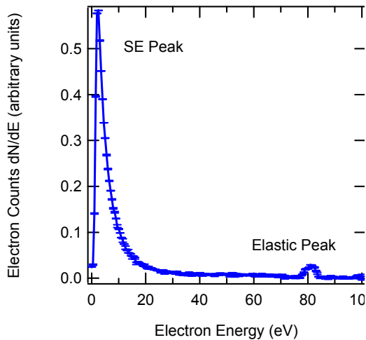
FIG. 1. Electron energy spectrum for Au, induced from a 80 eV electron beam. SE peak at 2.3 \pm 0.5 eV.
