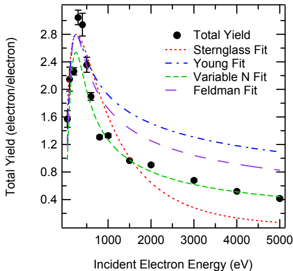
FIG. 10. In contrast to Fig. 8, reliable absolute total yields were obtained with flooding the sample between yield measurements. This yield curve for Al2219 (5 \mu s pulses with amplitudes 50 nA, each data point was the average of 10 pulses) is fitted with various analysis models. Best estimates for yield parameters are provided in Table 3.
