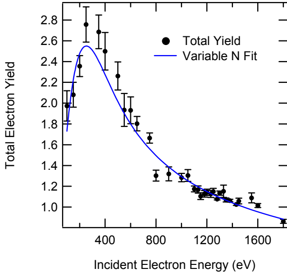
FIG. 11. Pulsed-yield curve versus beam energy for CV-1147 sample 1 with flood gun neutralization after each pulse. Each yield point was the average of 10 pulsed-yield measurements ( 5 \mu\text{s} pulse with amplitude 50 nA) with standard errors as the error bars. The best model estimates for the total yield parameters were: \sigma_{\text{max}}=2.5\pm 0.1 at E_{\text{max}}=250\pm 10 eV, E_1=40\pm 20 eV, and E_2=1470\pm 40 eV. Model estimates for the maximum yield were low compared to the data.
