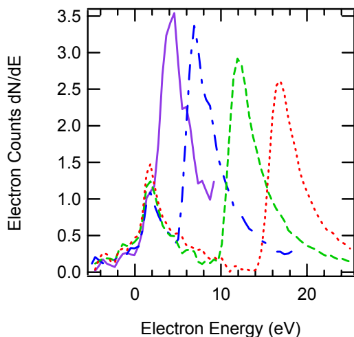
FIG. 3. SE spectra on negatively biased gold for -2 V (solid), -5 V (dash-dot), -10 V (short dash), and -15 V (dot). Measured with respect to the grounded grid peak (1.8 eV), the SE peak positions correspond to the applied potentials, accurate to \pm 1 eV.
