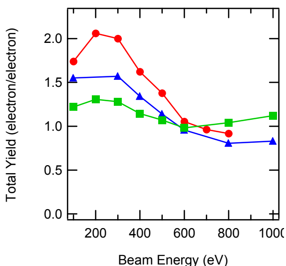
FIG. 8. Three consecutive yield curves for Al2219. Each data point consists of one pulse ( \sim 10^6 electrons/pulse). No neutralization methods were used. The first ( \bullet ), second ( \blacktriangle ), and third ( \blacksquare ) yield curves quickly flatten towards unity as the sample charged.
