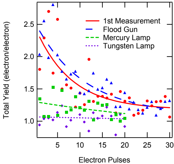
FIG. 9. Dampening of total yields at 500 eV as a function of electron pulses (5 \mu s pulses with amplitude 50 nA) for Al2219, along with exponential fits. First yield sequence (●) and sequence following electron flooding (▲) produced similar yield decay curves indicating that flooding discharged the sample effectively. Yield sequences following mercury (■) and tungsten filament (◆) lamp irradiation remained close to unity, indicating ineffective neutralization.
