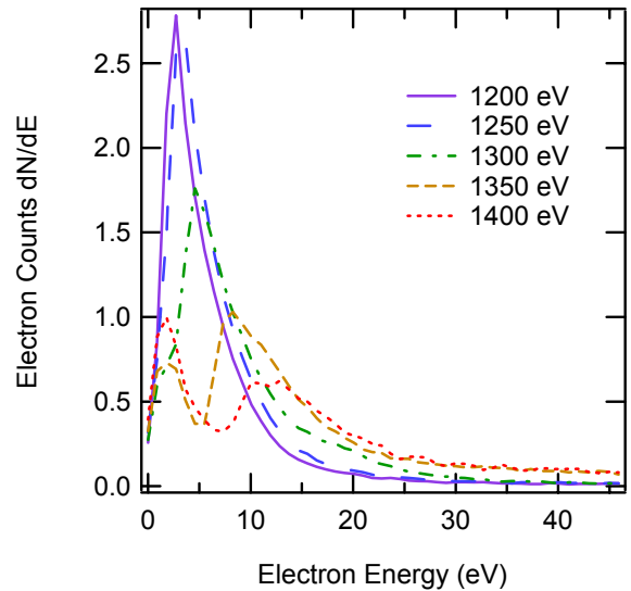
FIG. 14. Shown are evolving SE spectra for sample 6 for increasing incident electron beam energies of 1200 eV (solid), 1250 eV (long dash), 1300 eV (dash-dot), 1350 eV (short dash), and 1400 eV (dot). These spectra indicated a crossing of E_2 at 1250-1300 eV.
