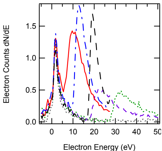
FIG. 6. SE DC spectra of Al2219 showed increasingly negative surface potentials at beam energies of 200 eV ( 9 \pm 1 V) (solid), 500 eV ( 11 \pm 1 V) (dash-dot), 1000 eV ( 17 \pm 1 V) (long dash), 1250 eV ( 21 \pm 2 V) (short dash), 1300 eV ( 32 \pm 2 V) (dot). Decline of SE peak magnitude at 1250 eV indicated dielectric breakdown once more at a surface potential of 21 \pm 2 V.
