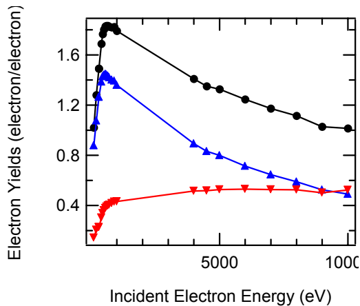
FIG. 2. Total ( \bullet ), SE ( \blacktriangle ), and BSE ( \blacktriangledown ) electron yields for Au as a function of incident electron beam energy. Total yield parameters are \sigma_{\max} = 1.8 \pm 0.1 at E_{\max} = 600 \pm 50 eV.
