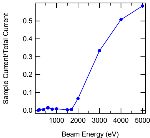
FIG. 5. Monitoring Al2219 sample current confirmed dielectric breakdown at 1600 eV, where the sample began to conduct DC current.
