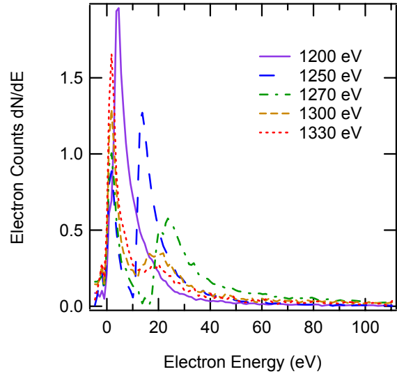
FIG. 13. Shown are evolving SE spectra for sample 1 for increasing electron beam energies of 1200 eV (solid), 1250 eV (long dash), 1270 eV (dash-dot), 1300 eV (short dash), and 1330 eV (dot). The emergence and right-shifting trend of the 2 nd SE peak was caused by a negative sample potential caused by the incident electron beam energy exceeding E_2 . These spectra indicated a crossing of E_2 at 1200-1250 eV.
