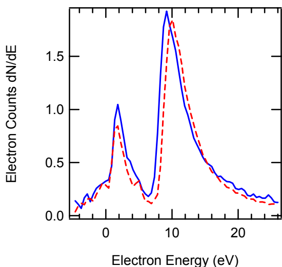
FIG. 7. DC-Spectra taken at 500 eV (solid) and 1000 eV (dash) after 5 keV irradiation on Al2219 showed “locked” negative surface potential of 7-9 V resulting from imbedded electron charge.
