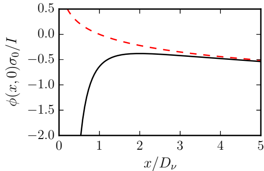
FIG. 2. The solid line represents the dependence of the 2D electric potential \phi(\mathbf{r}) on x/D_\nu for a viscous 2D electron system confined to a half plane. The potential is measured in units of I/\sigma_0 and is evaluated at the edge of the system, i.e., at y = 0 . The Ohmic result in the absence of viscosity is also plotted (dashed line). We clearly see that viscosity introduces a region \sim 2D_\nu near the injector where the 2D electrical potential is large and negative.
