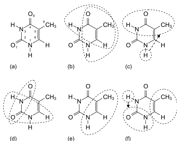
Fig. 4. (a) Structure of the thymine molecule, (b)–(f) possible dissociation processes of the core-ionized thymine molecule. The encircled regions show possible assignments of the observed positive ions (see text for more details): (b) 83 u, (c) 71 u, (d) 70 u, (e) 55 u, and (f) 44 u (left) and 40 u (right).
