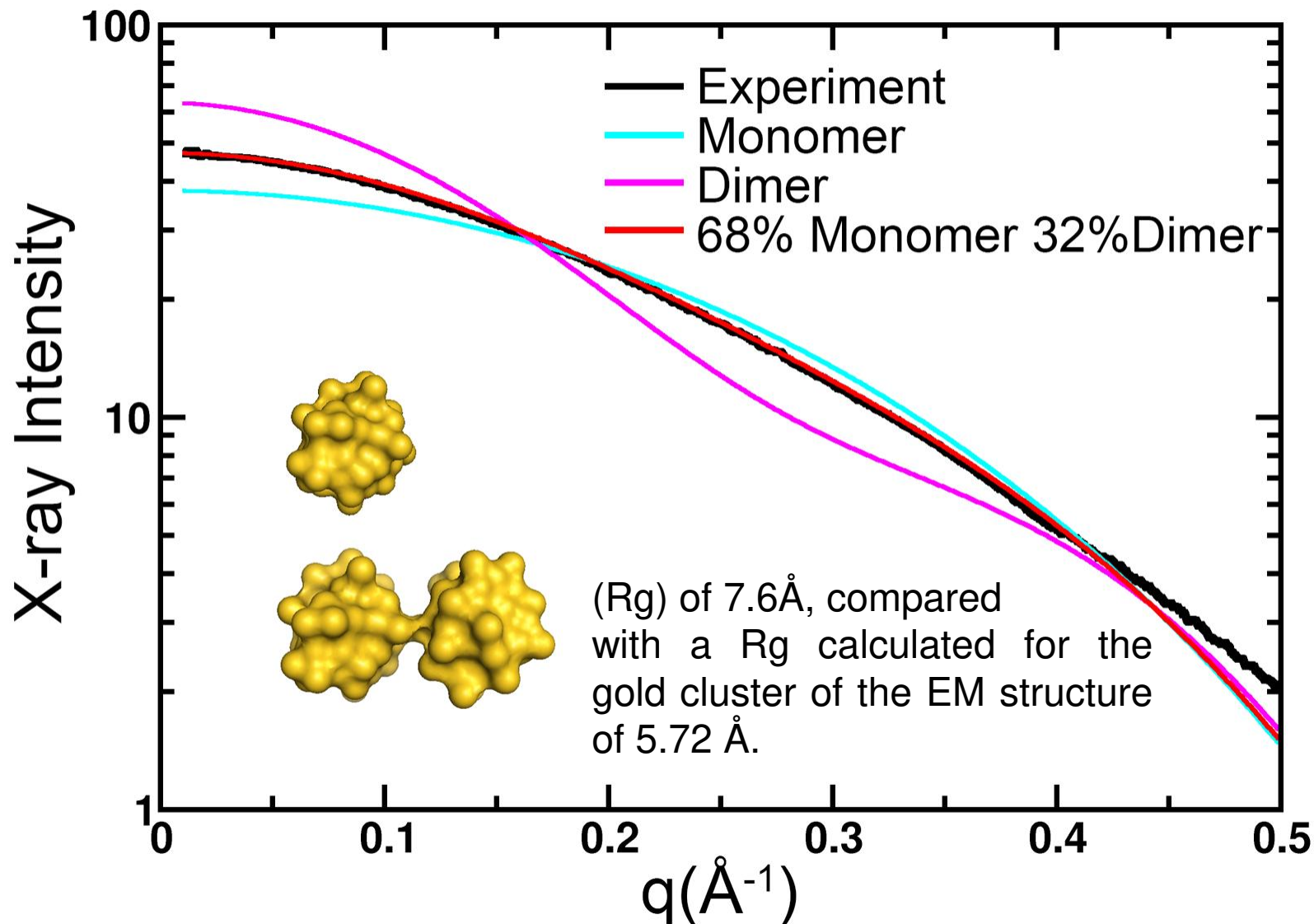
Small angle X-ray scattering (SAXS) from Au 68 NPs. Using atomic coordinates of monomers and modeled dimers (bottom inset) the calculated SAXS profiles were compared against experiment. A mixture (red) with a major population of monomer (cyan) and minor population dimer (magenta) had a best fit.
