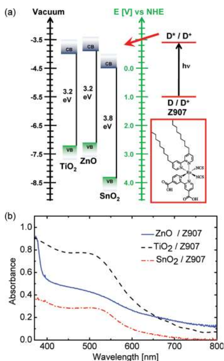
Figure 1. (a) Schematic diagram illustrating the energy levels of the conduction band (CB) and valence band (VB) of \text{TiO}_2 , \text{ZnO} , and \text{SnO}_2 as taken from refs 2–5. Also shown is the approximate redox potential of ground and excited states of Z907 ruthenium-based dye 18 (molecular structure shown in inset). The red arrow indicates electron injection from the dye LUMO states into the respective metal-oxide CB. (b) Steady-state absorption spectra measured for sensitized nanoporous films of \text{ZnO} (blue solid line, film thickness 0.6 \mu\text{m} ), \text{SnO}_2 (red dash-dot line, film thickness 1 \mu\text{m} ), and \text{TiO}_2 (black dashed line, film thickness 3 \mu\text{m} ) using an integrating sphere. Spectra were taken for film samples used in the terahertz photoconductivity measurements, and these data were used to calculate the terahertz effective mobility \phi_{\text{inj}}^{\mu\text{THz}} . We note that the films used for the solar cells below are much thicker and therefore display a higher optical density ( \text{OD} > 2 ) at the absorption maximum. Details of film preparation and thicknesses are given in the Materials and Methods section.
