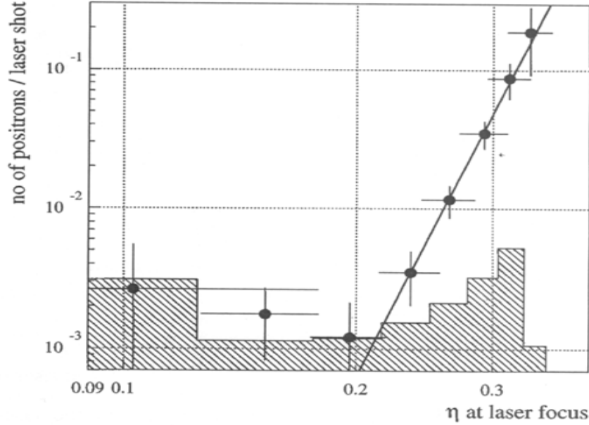
Figure 13: Dependence of the positron rate per laser shot on the laser field-strength parameter \eta . The line shows a power law fit to the data. The shaded distribution is the 95% confidence limit on the residual background from showers of lost beam particles after subtracting the laser-off positron rate. This figure is reproduced from Fig. 4 in Ref. [39]
