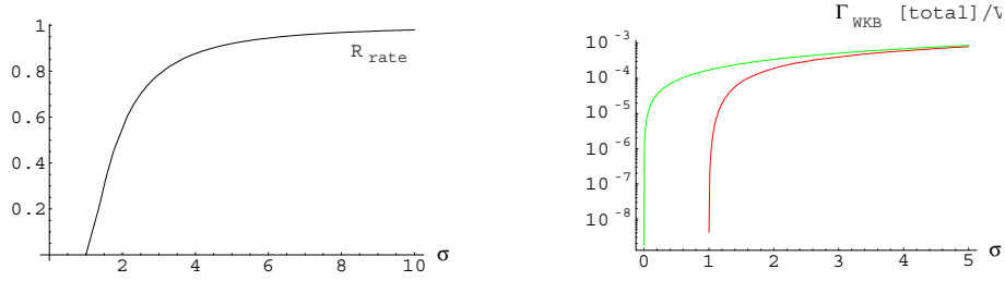
Figure 8: Left: Ratio R_{\text{rate}} defined in Eq. (317) is plotted as function of \sigma_s in the left figure. Right: Number of pairs created in slab of Compton width per area and time as functions of \sigma_s . Upper curve is for the constant field (295), lower for the Sauter field (308)). Both plots are for E_0 = E_c and \sigma_s = \ell/\lambda_C .
