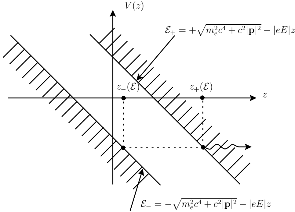
Figure 4: Energy-spectra \mathcal{E}_{\pm} with an external electric field \mathbf{E} along \hat{\mathbf{z}} -direction (for -\ell < z < \ell and \ell \gg 1 ). Crossing energy-levels appear, indicated by a dashed line between two continuum energy-spectra \mathcal{E}_{-} and \mathcal{E}_{+} . The turning points z_{\pm}(\mathcal{E}) for the crossing energy-levels \mathcal{E} of Eq. (51) are marked. This implies that virtual electrons at these crossing energy-levels in the negative energy-spectrum can quantum-mechanically tunnel toward infinity [ z \gg z_{+}(\mathcal{E}) ] as real electrons; empty states left over in the negative energy-spectrum represent real positrons. This is how quantum tunneling produces pairs of electrons and positrons.
