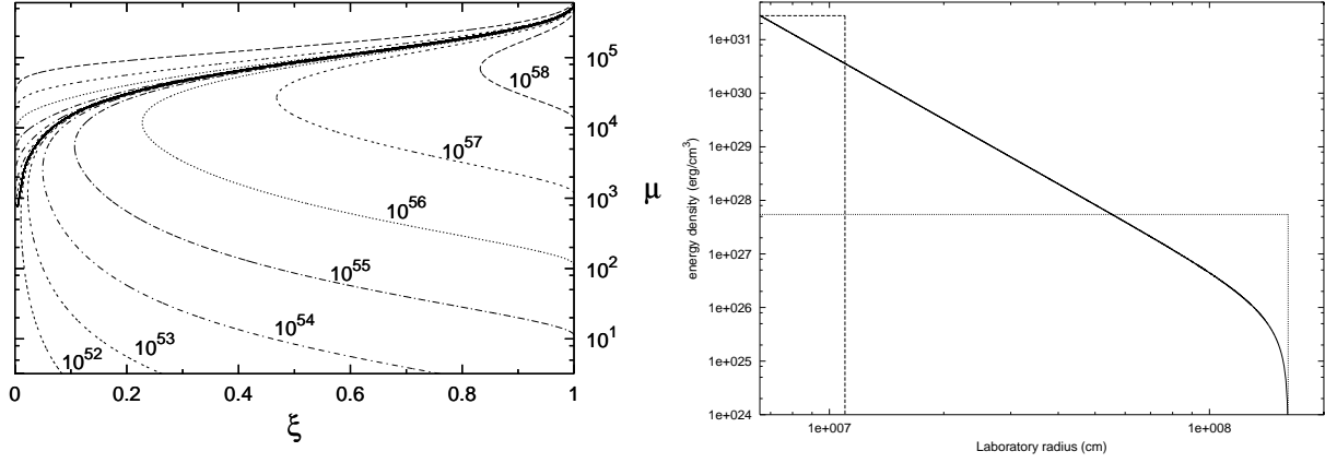
Figure 21: Left) Selected lines corresponding to fixed values of the \mathcal{E}_{\text{dya}} are given as a function of the two parameters \mu \xi , only the solutions below the continuous heavy line are physically relevant. The configurations above the continuous heavy lines correspond to unphysical solutions with r_{\text{ds}} < r_+ . Right) There are two different approximations for the energy density profile inside the Dyadosphere. The first one (dashed line) fixes the energy density equal to its peak value, and computes an “effective” Dyadosphere radius accordingly. The second one (dotted line) fixes the Dyadosphere radius to its correct value, and assumes a uniform energy density over the Dyadosphere volume. The total energy in the Dyadosphere is of course the same in both cases. The solid curve represents the real energy density profile. Details in [404].
