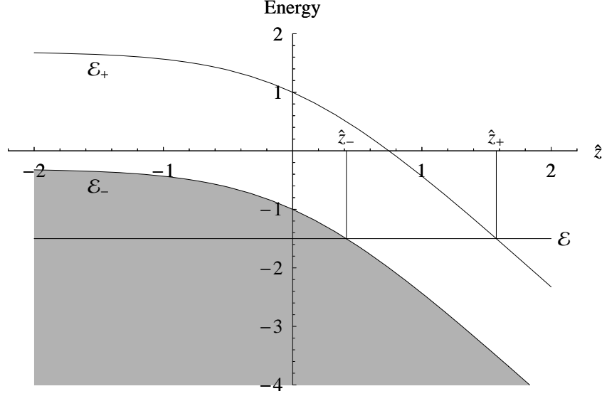
Figure 9: Energies (246) for a soft electric field step E(z) of Eq. (318) and the potentials V_{\pm}(z) (318) for \sigma_s = 5 . Positive and negative-energies \mathcal{E}_{\pm}(z) of Eq. (246) are plotted for p_z = p_{\perp} = 0 as functions of \hat{z} = z/\ell .
