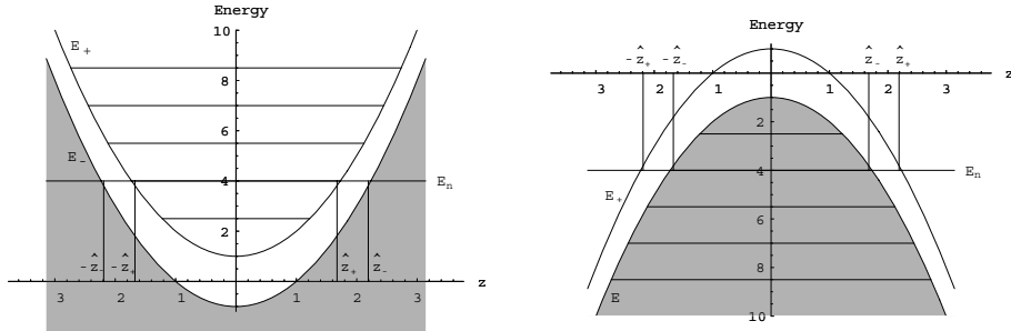
Figure 10: Positive- and negative-energy spectra \mathcal{E}_{\pm}(z) of Eq. (246) for p_z = p_{\perp} = 0 as a function of \hat{z} \equiv z/\lambda_C for the linearly rising electric field E(z) with the harmonic potential (328). The reduced field strengths are \epsilon = 2 (left figure) and \epsilon = -2 (right figure). On the left, bound states are filled and positrons escape to z = \pm\infty . On the right, bound electrons with negative energy tunnel out of the well and escape with increasing energy to z = \pm\infty .
