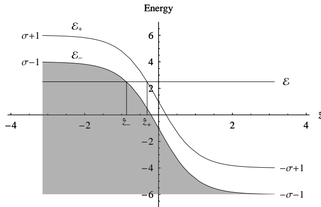
Figure 6: Positive- and negative-energy spectra \mathcal{E}_{\pm}(z) of Eq. (246) in units of m_e c^2 , with p_z = p_{\perp} = 0 as a function of \hat{z} = z/\ell for the Sauter potential V_{\pm}(z) (297) for \sigma_s = 5 .
