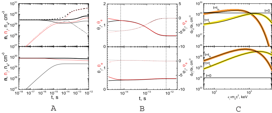
Figure 41: A: Dependence on time of concentrations of pairs (black), photons (red) and both (thick) when all interactions take place (solid). Upper (lower) figure corresponds to the case when initially there are mainly pairs (photons). Dotted curves on the upper figure show concentrations when inverse triple interactions are neglected. In this case an enhancement of the pairs occurs with the corresponding increase in photon number and thermal equilibrium is never reached. B: Time dependence of temperatures, measured on the left axis (solid), and chemical potentials, measured on the right axis (dotted), of electrons (black) and photons (red). The dashed lines correspond to the reaching of the kinetic ( \sim 10^{-14} sec) and the thermal ( \sim 10^{-12} sec) equilibria. Upper (lower) figure corresponds to the case when initially there are mainly pairs (photons). C: Spectra of pairs (upper figure) and photons (lower figure) when initially only pairs are present. The black curve represents the results of numerical calculations obtained successively at t = 0 , t = t_k and t = t_{th} (see the text). Both spectra of photons and pairs are initially taken to be flat. The yellow curves indicate the spectra obtained from (657) at t = t_k . The perfect fit of the two curves is most evident in the entire energy range leading to the first determination of the temperature and chemical potential both for pairs and photons. The orange curves indicate the final spectra as thermal equilibrium is reached.
