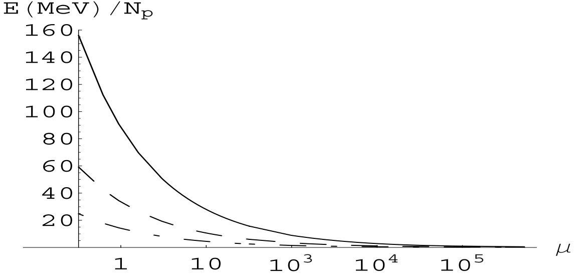
Figure 20: The average energy per pair is shown here as a function of the black hole mass in solar mass units for \xi = 1 (solid line), \xi = 0.5 (dashed line) and \xi = 0.1 (dashed and dotted line).
