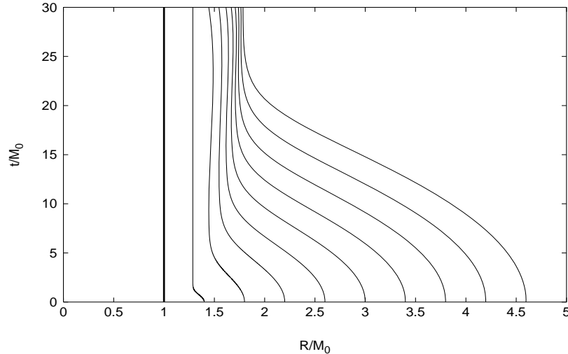
Figure 27: Collapse curves for neutral shells with rest mass M_0 starting at rest at selected radii R^* computed by using the exact solutions given in Ref. [405]. A different value of M_{\text{irr}} (and therefore of r_+ ) corresponds to each curve. The time parameter is the Schwarzschild time coordinate t and the asymptotic behaviour at the respective horizons is evident. The limiting configuration M_{\text{irr}} = \frac{M_0}{2} (solid line) corresponds to the case in which the shell is trapped, at the very beginning of its motion, by the formation of the horizon.
