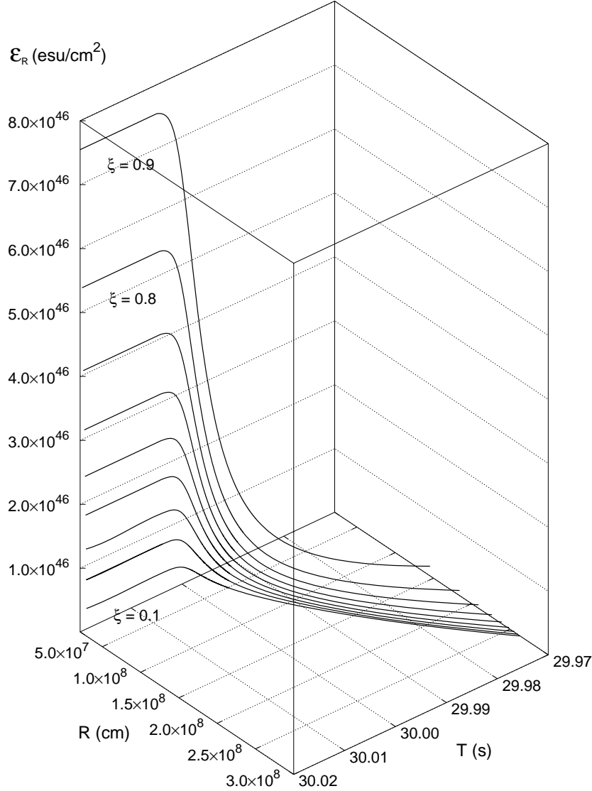
Figure 26: Electric field behaviour at the surface of the shell for M = 20M_{\odot} and for different values of the parameter \xi . The asymptotic behavior is the clear manifestation of general relativistic effects as the horizon of the black hole is approached. Details in [405].
