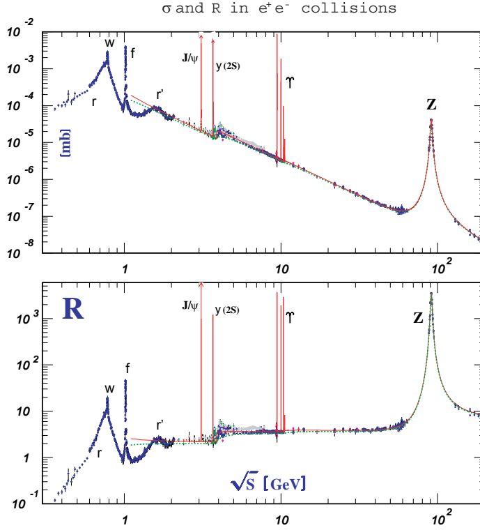
Figure 11: The total cross section of e^+e^- \rightarrow \text{hadron} (346) and the ratio R = \sigma_{e^+e^- \rightarrow \text{hadron}} / \sigma_{e^+e^- \rightarrow \mu^+\mu^-} (347), where s \equiv q_{\text{cm}}^2 . Reproduced from Ref. [C. Amsler et al. (Particle Data Group), Physics Letters B667, 1 (2008)].
