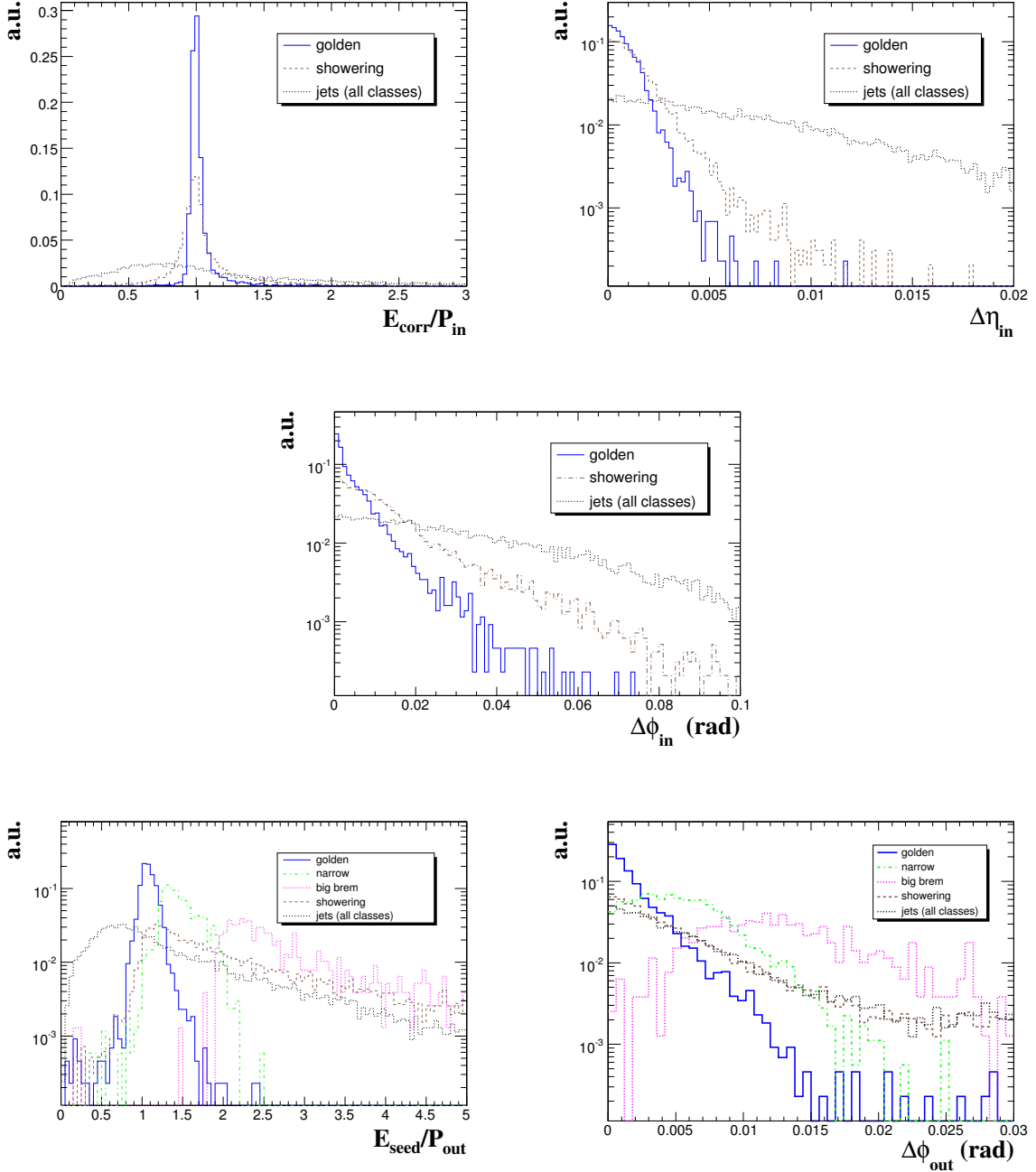
Figure 24: Distributions of electron identification observables in the \eta range of the ECAL barrel. The distributions of track-cluster matching observables are shown for different classes of electrons, and in comparisons with distributions for “fake” electron candidates from QCD jet background. Similar distributions with larger spread are obtained for electrons in the endcaps.
