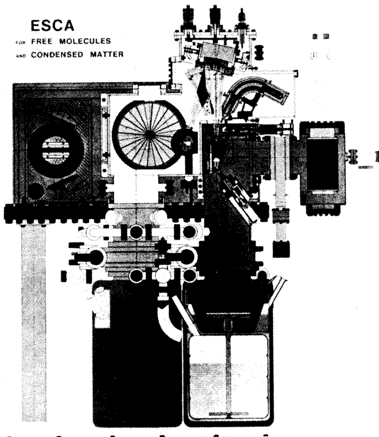
Fig. 16. Side view of the new ESCA instrument for free molecules and condensed matter. The instrument is UHV compatible and includes four different excitation modes (Monochromatized AlK\alpha ; Monochromatized and polarized UV; electron impact; monochromatized electron impact).
