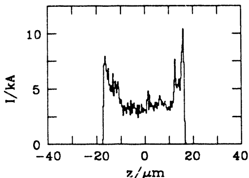
Fig. 5. The bunch shape for the example of Fig. 4 except that after the 2 nd compression particles with energy deviations \delta > 2.0\% and \delta < -1.5\% are removed.
