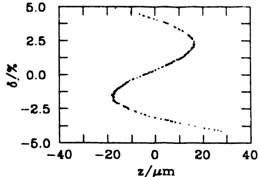
Fig. 3. Phase space after the 2 nd compression. The bunch head points to negative values of z .
