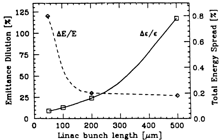
Fig. 1 Transverse emittance dilution (solid) and peak-to-peak energy spread (dashed) as a function of the linac bunch length. The emittance dilution is in units of the initial emittance \gamma\epsilon_{x,y} = 3 mm-mrad and the energy spread is in percent with a scale on the right. The plotting symbols are the values calculated.
