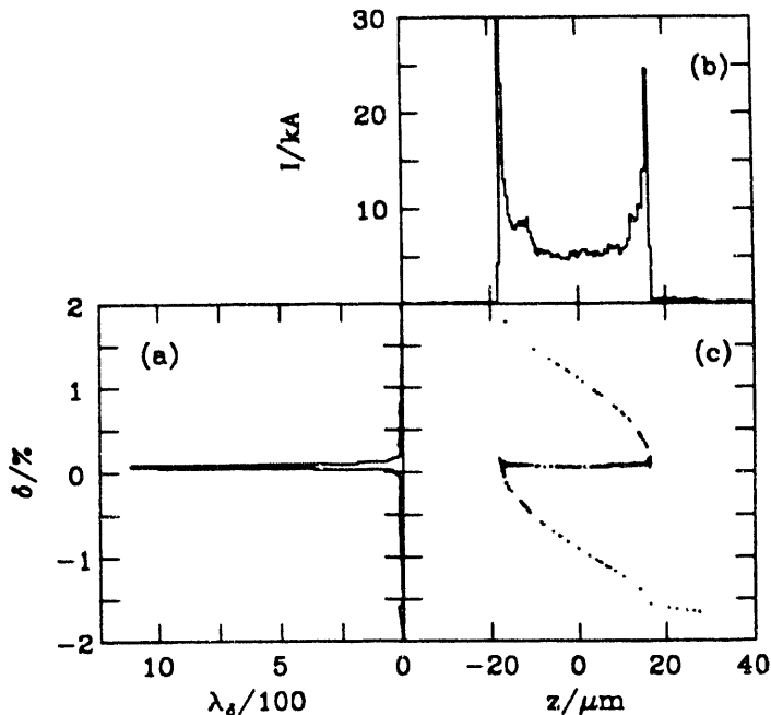
Fig. 4. The energy spectrum (a), the charge distribution (b), and the shape of phase space (c) at the end of the linac.
