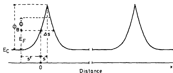
FIG. 1. Energy band diagram of heavily-doped polycrystalline CdS.
