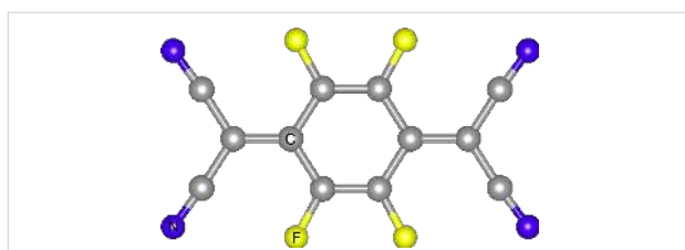
Figure 4: Molecular geometry of tetrafluorotetracyanoquinodimethane ( F_4 -TCNQ).
