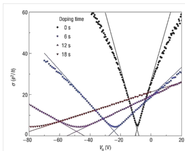
Figure 2: Conductivity as a function of the gate voltage ( \sigma(V_{\text{g}}) ) of graphene at different exposures to K. The shift of neutrality point to negative gate voltages indicates an increase of n-type doping with increasing exposure to K atoms. The change in the slope of the curves suggest a reduction of the mobility of the charge carriers. Reprinted with permission from [29]. Copyright 2008 Nature Publishing Group.
