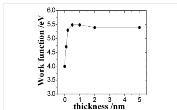
Figure 5: Plot of the workfunction of graphene (eV) as a function of the thickness (nm) of deposited F_4 -TCNQ. The workfunction of graphene increases 1.3 eV after the deposition of 0.2 nm of F_4 -TCNQ. For higher thicknesses the workfunction remains constant suggesting that the charge transfer occurs at the graphene/ F_4 -TCNQ interface. Reprinted with permission from [35]. Copyright 2007 American Chemical Society.
