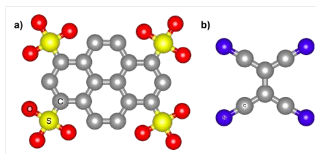
Figure 6: Molecular structure of a) pyrenetetrasulfonic acid (TPA) and b) tetracyanoethylene (TCNE).
