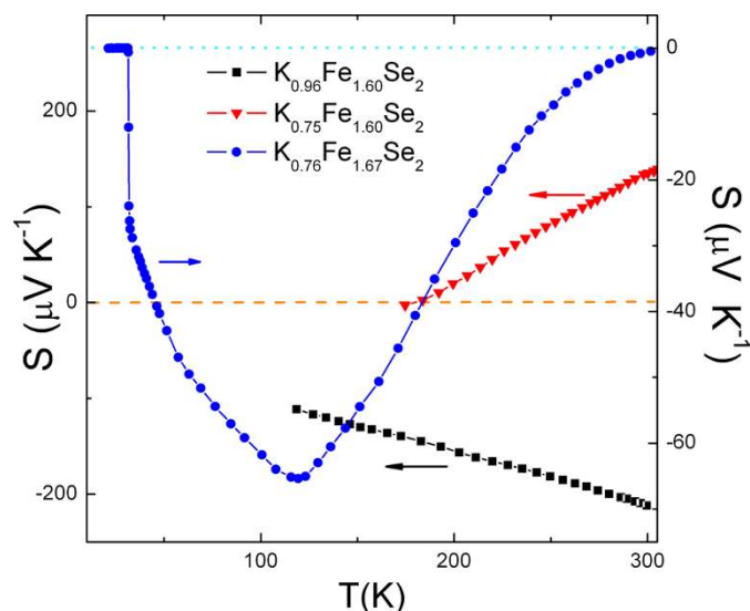
Figure 2 | Typical Seebeck coefficient as a function of temperature for the samples in the three regions of the phase diagram. Region I: K_{0.75}\text{Fe}_{1.6}\text{Se}_2 ; Region II: K_{0.76}\text{Fe}_{1.67}\text{Se}_2 ; Region III: K_{0.96}\text{Fe}_{1.60}\text{Se}_2 .
