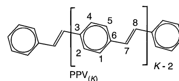
Fig. 1. Geometry and atom labeling of PPV oligomers. Bond angles are 120^\circ , except \alpha(r_{6,7}, r_{7,8}) = 128^\circ , and the distances are r_{1,2} = r_{2,3} = r_{3,4} = r_{4,5} = r_{5,6} = r_{6,1} = 1.39 \text{ \AA} , r_{6,7} = 1.44 \text{ \AA} , and r_{7,8} = 1.33 \text{ \AA} .
