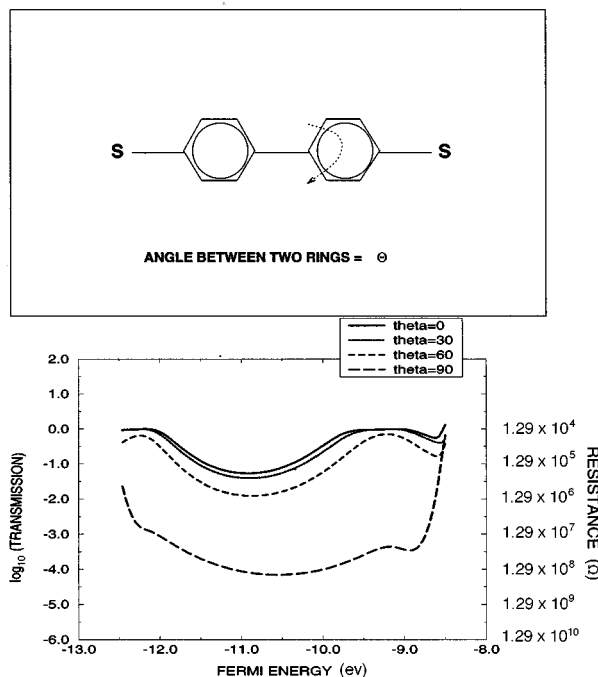
FIG. 6. Transmission function (and resistance) vs Fermi energy for molecules with successive benzene rings misaligned by different angles \theta . As \theta increases from 0^\circ to 90^\circ , transmission goes down (resistance goes up) due to decrease in overlap between the \pi orbitals in the rings. Log scale in the plot represents decimal log.
