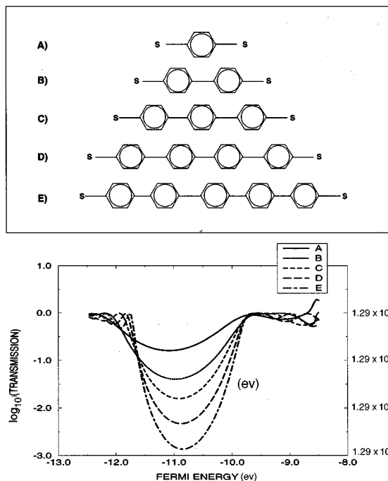
FIG. 5. Transmission function (and resistance) vs Fermi energy for molecules with different numbers of benzene rings. Transmission goes down exponentially (resistance goes up) as the number of benzene rings is increased. Log scale in the plot represents decimal log.
