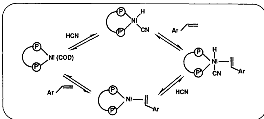
Fig. 9. Hydrocyanation mechanism I.
