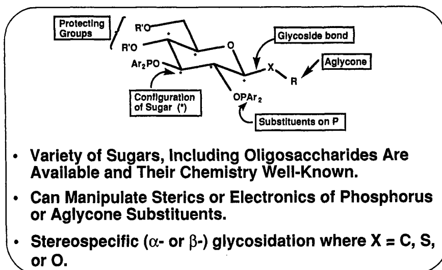
Fig. 2. Design of 1,2-diol phosphinite ligands from sugars.
