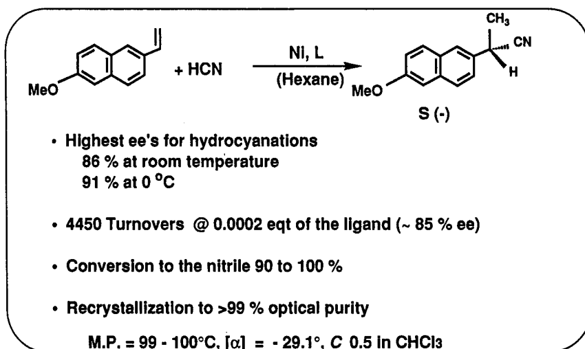
Fig. 6. Synthesis of naproxen nitrile.
