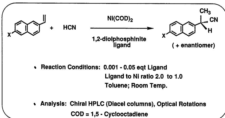
Fig. 4. The protocol for the Ni(0)-catalyzed hydrocyanation of vinylarenes.
