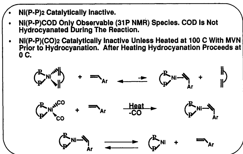
Fig. 7. Summary of some mechanistic studies.
