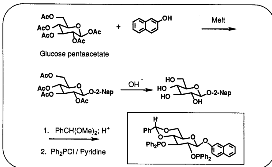
Fig. 3. Synthesis of prototypical sugar diol phosphinites.
