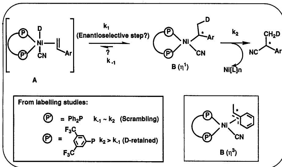
Fig. 10. Hydrocyanation mechanism II.
