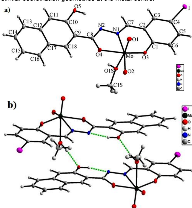
Fig. 1. a) The structure of complex [\text{MoO}_2(\text{L}^{1\text{a}})(\text{CH}_3\text{OH})] ( 1 ) with the atom numbering scheme. Displacement ellipsoids are drawn at the 30% probability level; b) Dimeric unit formed by intermolecular hydrogen bonding in complex 1 . Hydrogen bonds are shown as green dashed lines (see Tables S1 and S2 for selected bond distances and angles).
