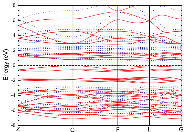
FIG. 2. Electronic band structure for majority (solid line) and minority (dot line) spin states of ferromagnetic LN-type MnTiO 3 phase along the high-symmetry directions in the Brillouin zone. The Fermi level is located at 0.0 eV.
