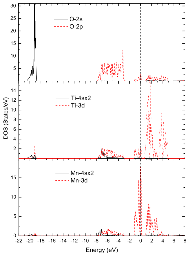
FIG. 1. Partial density of states of paramagnetic LN-type MnTiO 3 phase. Fermi energy is set to zero.
