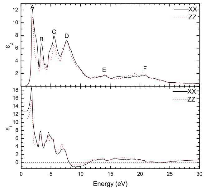
FIG. 4. The imaginary part \varepsilon_2(\omega) and real part \varepsilon_1(\omega) of the dielectric function of LN-type MnTiO 3 . The solid and dot lines represent the polarization direction of xx and zz, respectively.
