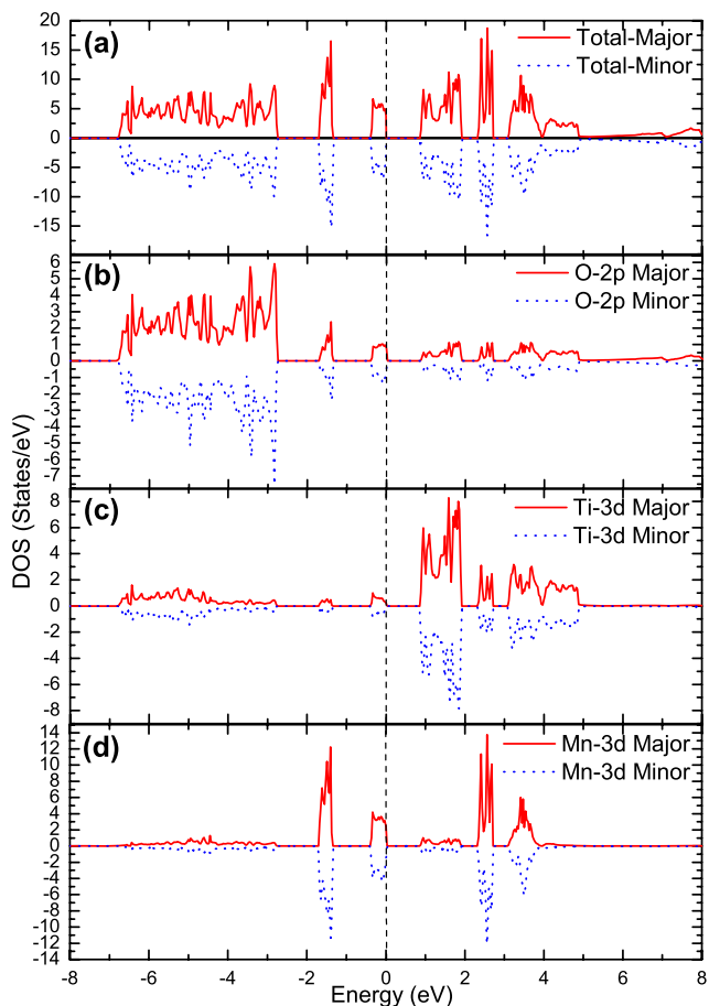
FIG. 3. Total electronic DOS (a) and the partial DOS of O 2p (b), Ti 3d (c), and Mn 3d (d) of G-antiferromagnetic LN-type MnTiO 3 , respectively. Majority and minority spins are shown above and below the axes, respectively. Fermi energy is set to zero.
