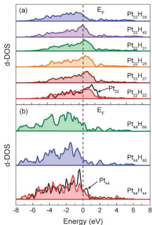
Fig. 8 DFT calculated d electron density of states (d-DOS) of unsupported and H-covered (a) \text{Pt}_{22}\text{H}_x ( x = 22, 27, 29, 31, 45, 59 ) and (b) \text{Pt}_{44}\text{H}_x ( x = 44, 60, 66 ).
