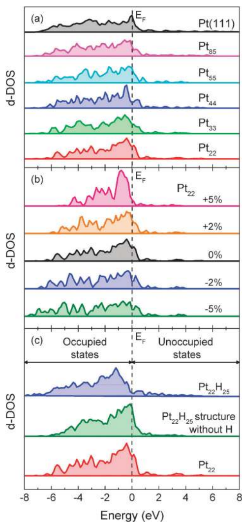
Fig. 7 (a) DFT calculated d-electron density of states (d-DOS) of unsupported clean \text{Pt}_x NPs ( x = 22, 33, 44, 55, 85 ) and of a Pt(111) surface. (b) Effect of compressive (–) and tensile (+) strain on the d-DOS of unsupported clean \text{Pt}_{22} . (c) Comparison of the d-DOS of clean unsupported \text{Pt}_{22} to \text{Pt}_{22}\text{H}_{25} and the same \text{Pt}_{22}\text{H}_{25} structure but after removing all hydrogen atoms without further lattice relaxation.
