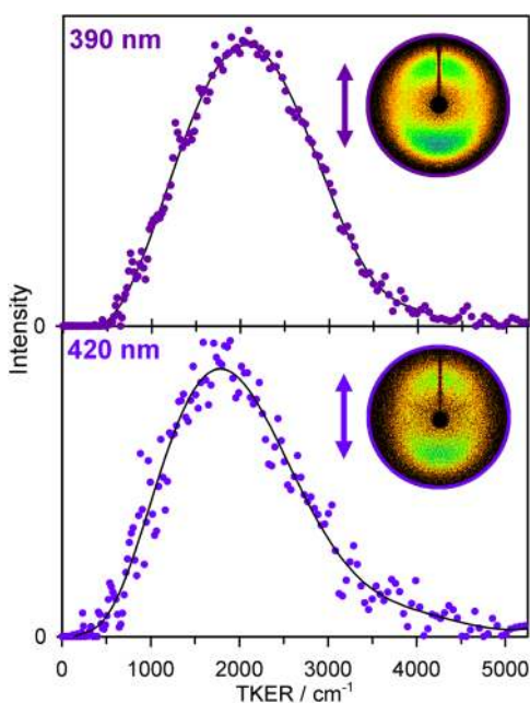
FIG. 7. Total kinetic energy release (TKER) distributions (points) and polynomial fits (line) for the O( 1 D) + MVK products obtained by velocity map imaging following UV-vis excitation of MVK-oxide at 390 nm (upper panel) and 420 nm (lower panel). Corresponding raw images of the O( 1 D) photoproducts are shown as insets. The blue double-sided arrows represent the polarization of the UV-vis OPO (parallel to the detector plane).
