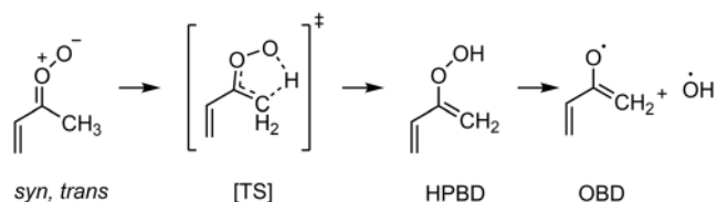
SCHEME 2. 1,4 H-atom transfer pathway for unimolecular decay of syn -MVK-oxide Criegee intermediate via HPBD to OH radical.
