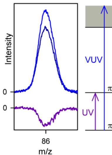
FIG. 4. Mass spectra ( m/z = 86 ) arising from photoionization of MVK-oxide with VUV radiation at 118 nm (10.5 eV). The top trace (blue) shows the photoionization signal. The middle trace (dark blue) shows the significant reduction ( \sim 20\% ) in the photoionization signal upon focused UV excitation at 390 nm (0.7 mJ/pulse) on the first \pi^* \leftarrow \pi transition, which results in ground state depletion. The lower trace (purple) shows the depletion signal (UV on–UV off). Also shown is a schematic energy level diagram indicating the \pi and \pi^* states and ionization limit (shaded) for the MVK-oxide Criegee intermediate.
