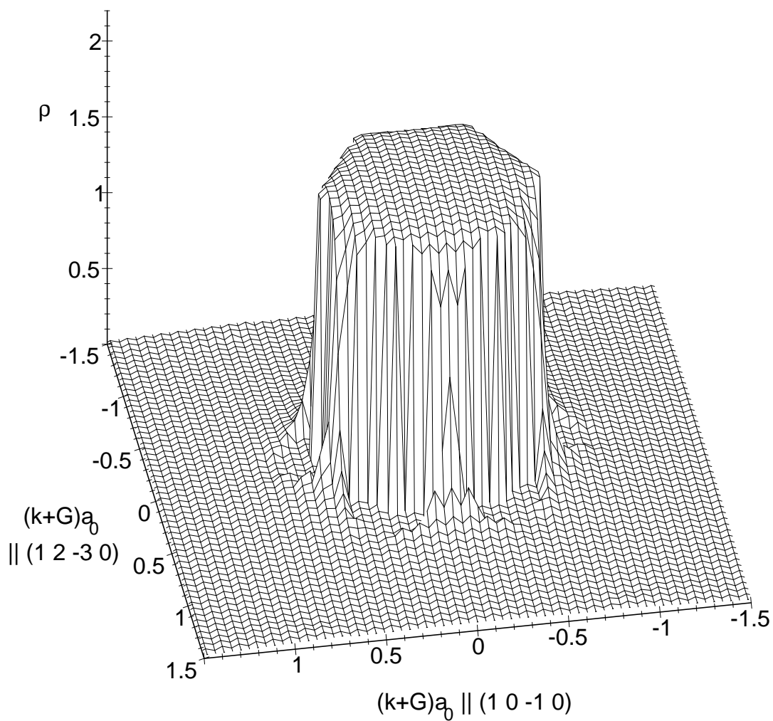
Fig. 3. The EMD [191] of hexagonal lithium as a function of \mathbf{k} + \mathbf{G} , which is varied in the plane spanned by (10\bar{1}0) and (12\bar{3}0) . Both momentum components are measured in units of 1/a_0 (reciprocal Bohr radii, atomic units). The relationship between the EMD and the Fermi surface has been discussed by Mearns and Kohn [192].
