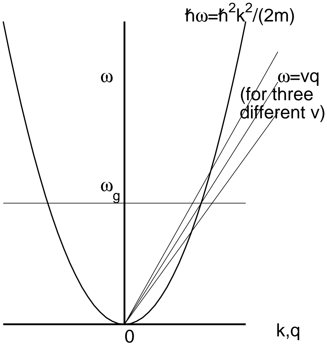
Fig. 10. The energy loss function has to be integrated over the triangular region Eq. (19), which simplifies for a homogeneous target to an integration over 0 \leq \omega \leq qv . The figure shows the upper left boundary of this region for three different v (in relationship to a gap \omega_g below, equal to, and above v_0 \sqrt{\hbar\omega_g/E_0}/2 with increasing slope) in form of three straight lines through the origin. E_0 is 1 rydberg.
