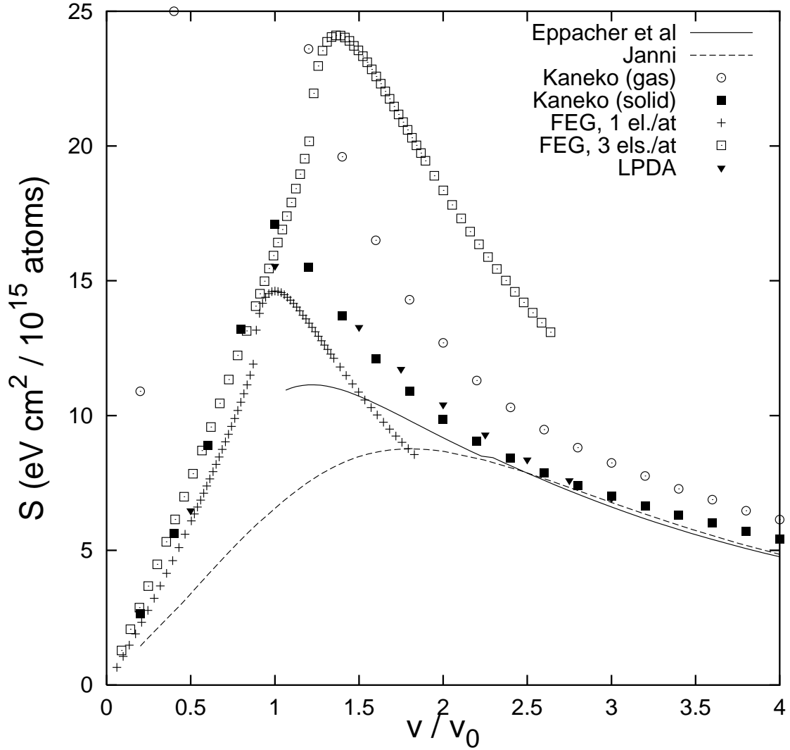
Fig. 9. Experimental proton stopping cross section of (probably bcc) Li by Eppacher et al. [195] and Janni [196], compared with calculated values for gaseous and solid Li from the Kaneko theory [15–17], and RPA free electron gas (FEG) values [10] with a homogeneous density equivalent to 1 or 3 electron(s) per Li atom (Fermi velocity 0.614v_0 or 0.885v_0 ) as shown. Values within the LPDA represent integrals of \rho(\mathbf{r}) of GTOFF Fitting Functions weighted with the Lindhard stopping number.
