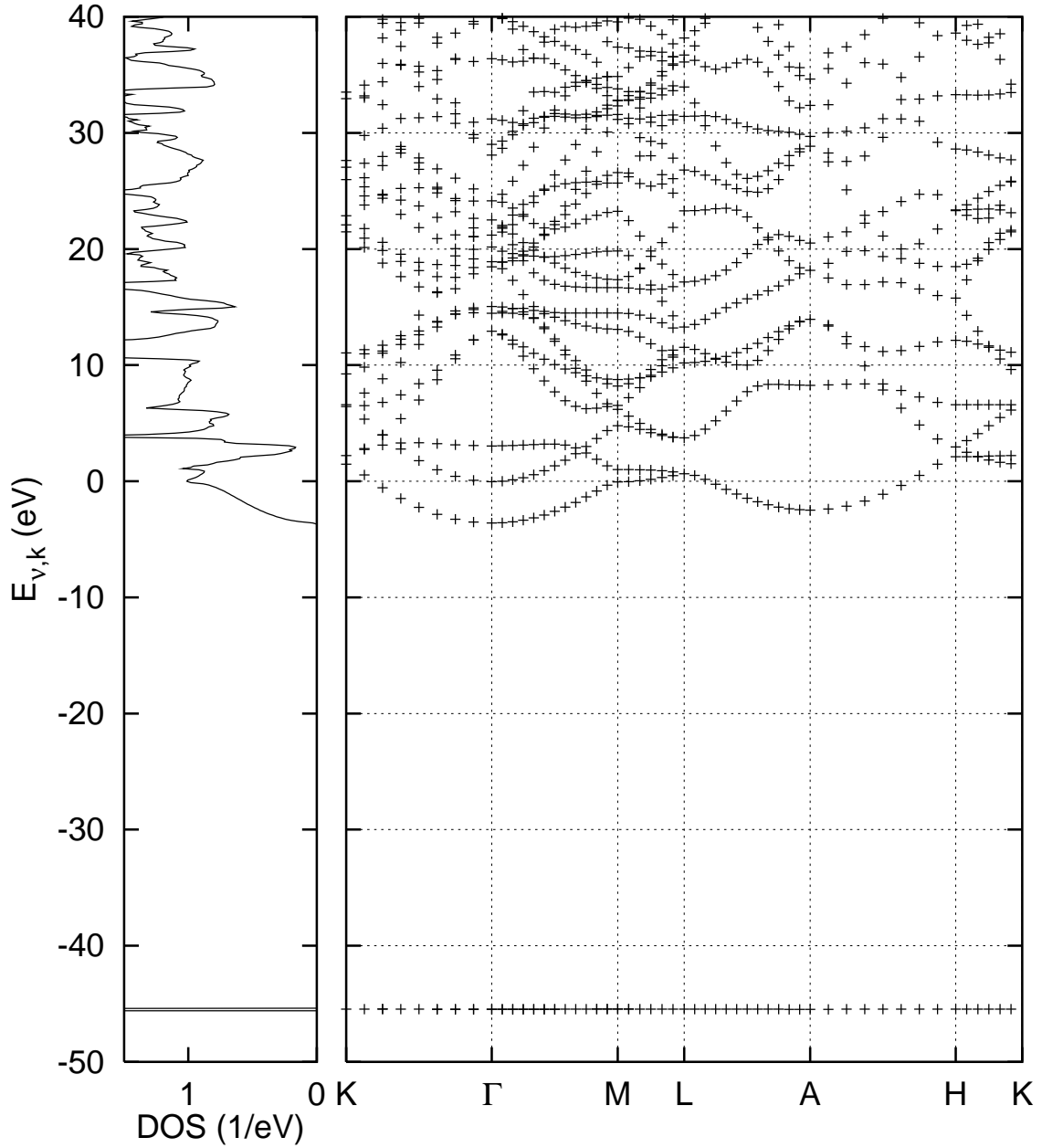
Fig. 1. Band-structure E_{\nu, \mathbf{k}} of hcp lithium at lattice parameters a = 5.65a_0 and c = 9.26a_0 [173] from GTOFF. E_F is set to 0 eV. This run used 24 \times 24 \times 12 \mathbf{k} -points in the BZ, that is 427 in the IBZ. The experimental value of the K -edge is about 10 eV lower than calculated here [189,190].
