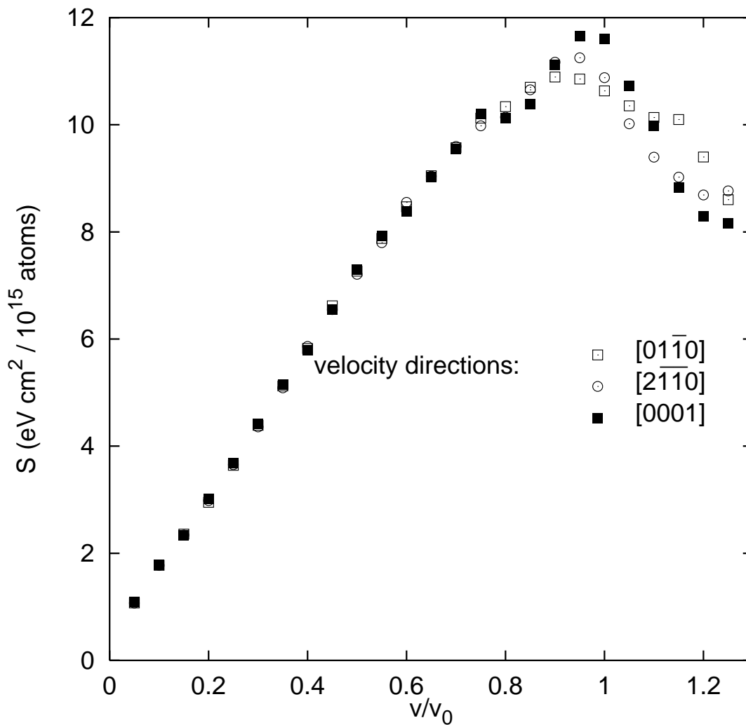
Fig. 8. Calculated lithium electronic stopping cross section. v_0 is the Bohr velocity. The energy loss function was integrated on a 27 \times 27 \times 33 mesh in \mathbf{q} -space (parallelepiped 5.6 \times 5.6 \times 5.4 a_0^{-3} ) and on a mesh with 64 points on the \omega -axis (0...87 eV). The lowest 24 bands were included in the sum over band-pairs in Eq. (7).
