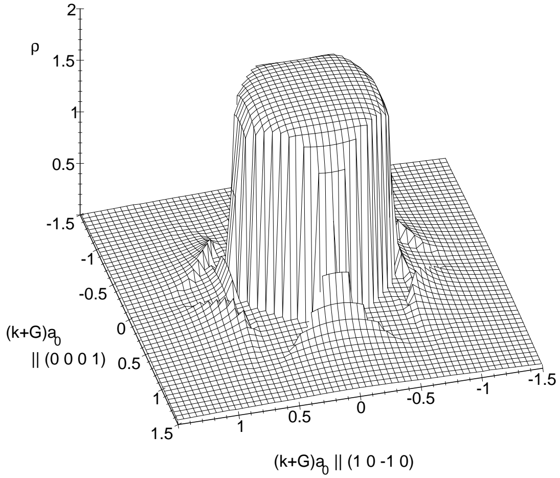
Fig. 4. The EMD of hexagonal lithium as a function of \mathbf{k} + \mathbf{G} , varied in the plane spanned by (10\bar{1}0) and (0001) . Where the BZ surfaces meet the Fermi surface, pieces are sheared off the Fermi ice block and drift as nearby floes. See [193,194] for the bcc phase.
