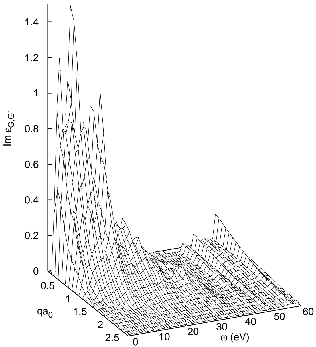
Fig. 6. \text{Im } \epsilon_{\mathbf{G},\mathbf{G}'} of hcp lithium for \mathbf{G} = \mathbf{G}' = (0001) , \mathbf{q} \parallel (10\bar{1}0) .
