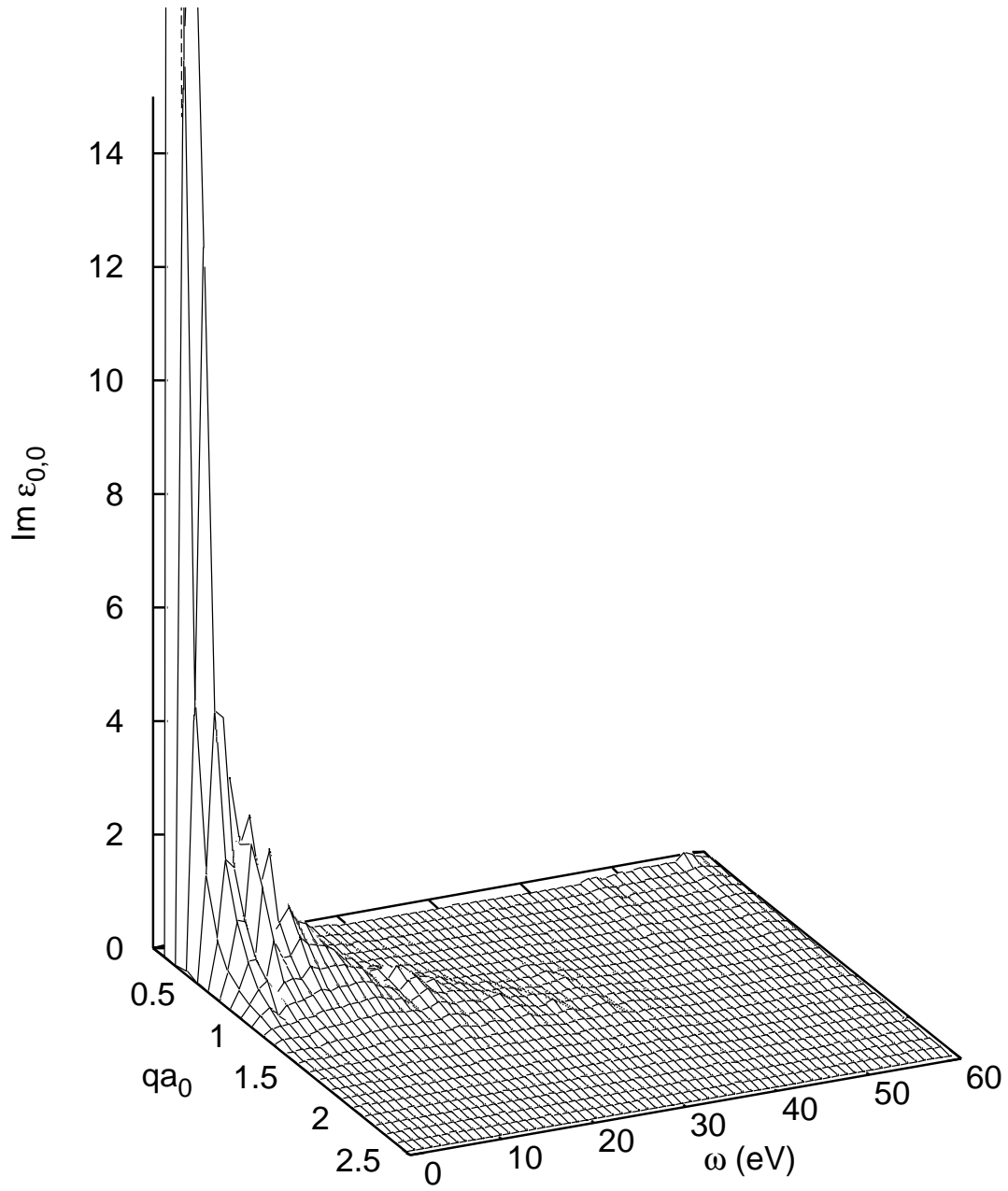
Fig. 5. Calculated \text{Im } \epsilon_{\mathbf{G},\mathbf{G}'} of hcp Li for \mathbf{G} = \mathbf{G}' = \mathbf{0} . \mathbf{q} \parallel (10\bar{1}0) . Figs. 5–7 have been calculated starting from a DFT input with 12 \times 12 \times 6 \mathbf{k} -points in the BZ (76 points in the IBZ).
