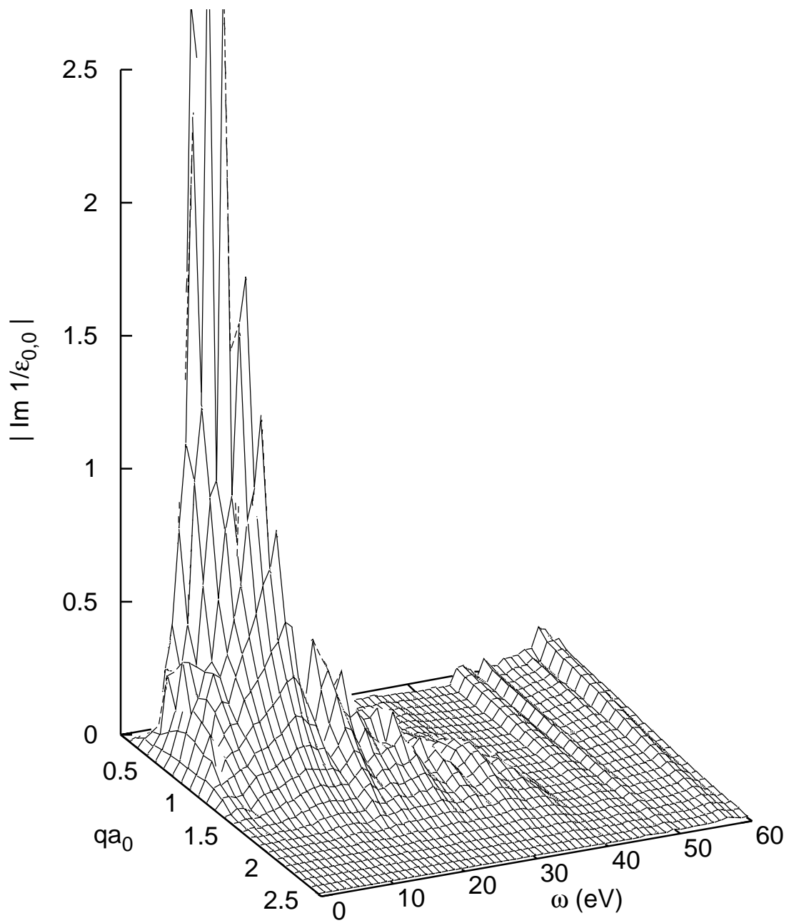
Fig. 7. Absolute value of \text{Im}[1/\epsilon_{0,0}(\mathbf{q}, \omega)] for hcp lithium. \mathbf{q} \parallel (10\bar{1}0) .
