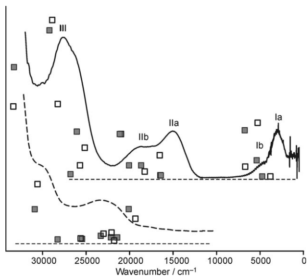
Figure 6. Electronic absorption spectra of \text{Fc}_2 (---) and \text{Fc}_2^{2+} (—) in Ar at 10 K. The filled squares (■) denote electronic transitions predicted by TD-BP86 calculations using the TZP basis set and the ZORA method as implemented in the ADF program, whereas the open squares (□) refer to calculations using the LANL2DZ basis set with the Gaussian program as listed in Tables 4 (for \text{Fc}_2 ) and 5 (for \text{Fc}_2^{2+} ).
