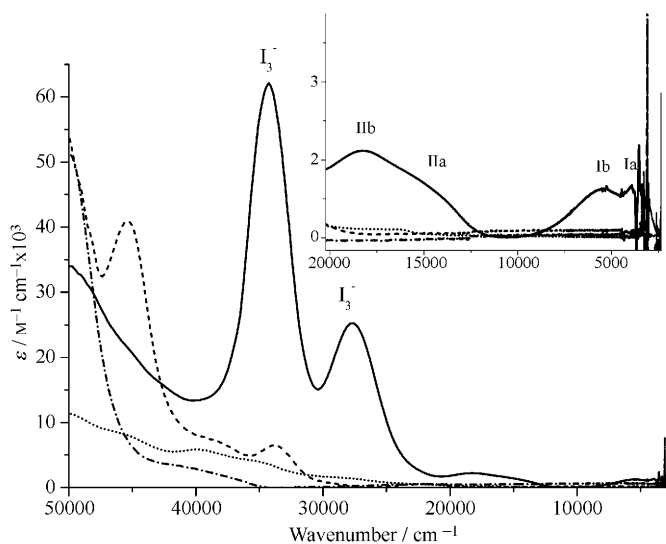
Figure 3. UV-visible-NIR-MIR spectra of biferrocenyl triiodide (Fc 2 I 3 ; —) along with those of the constituent subunits ferrocene (Fc; - - -) and ferrocenium hexafluorophosphate (FcPF 6 ; ····), and the neutral parent neutral compound biferrocene (Fc 2 ; - · - ·) in [D 3 ]acetonitrile.
