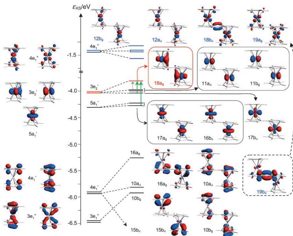
Figure 2. Kohn–Sham molecular orbitals of Fc (left-hand side) and Fc 2 (right-hand side) from BP86/DZ(ZORA) calculations with the ADF program. Blue levels are virtual MOs, red levels are open shells in the radical cations, and black levels are doubly occupied MOs. Dipole-allowed IR transitions are indicated by green arrows.
