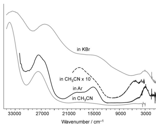
Figure 7. Comparison of optical absorption spectra of \text{Fc}_2^{2+} in KBr, \text{CH}_3\text{CN} (also multiplied by 10 for clarity), and an Ar matrix.
