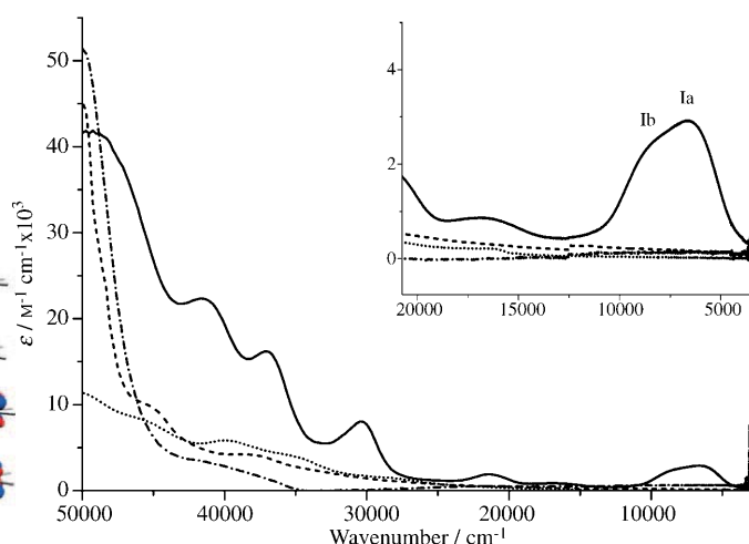
Figure 10. UV-visible-NIR-MIR spectra of Fc=FcPF 6 (—) along with those of the constituent subunits ferrocene (Fc; ---) and ferrocenium hexafluorophosphate (FcPF 6 ; ····) in acetonitrile and the neutral parent compound biferrocenylene (Fc=Fc; -·-·) in KBr, 300 K.
