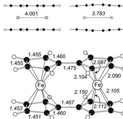
Figure 8. Structure of Fc=Fc and its radical cation, calculated by the BP86/LANL2DZ method, with interatomic distances [ \text{\AA} ] indicated in normal font for the neutral dimer and in italic for the radical cation.
