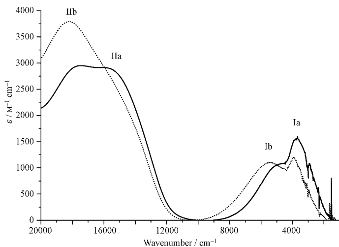
Figure 4. Low-energy bands of the 1',1'''-diethylbiferrocenyl triiodide (\text{FcEt})_2\text{I}_3 in dichloromethane (—) and in acetonitrile (.....), using a \text{CaF}_2 cell (300 K).
