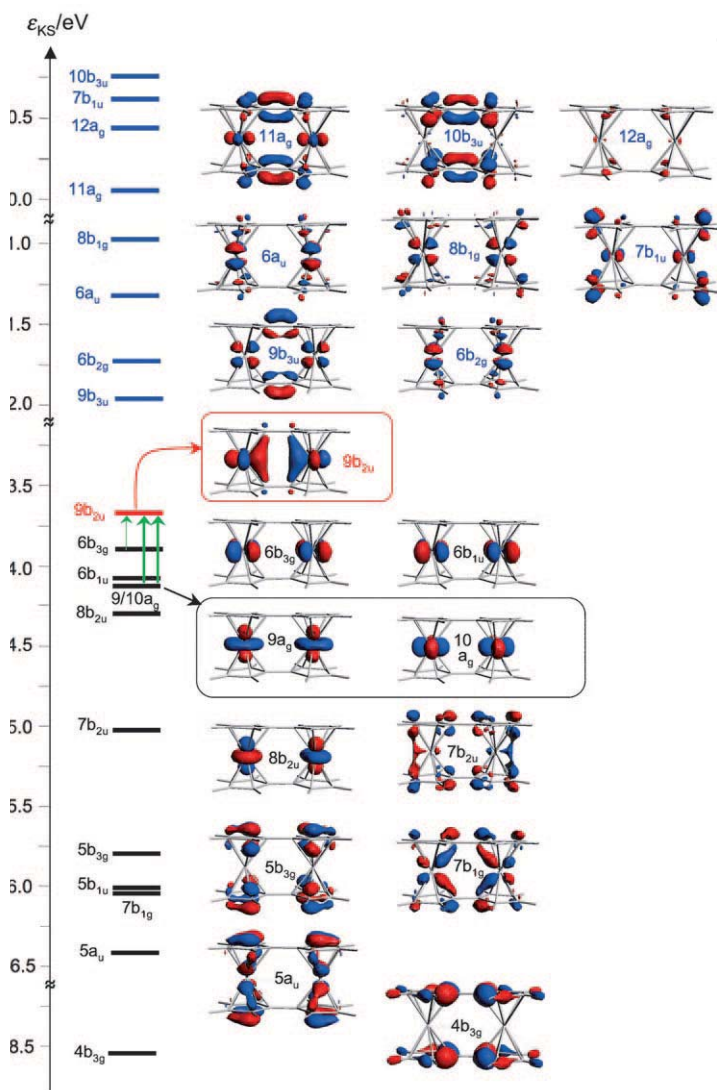
Figure 9. MO scheme of Fc=Fc from BP86/DZ(ZORA) calculations with the ADF program. Blue levels are virtual MOs, red levels are open shells in the radical cations, and black levels are the doubly occupied MOs. Dipole-allowed IR transitions are indicated by green arrows.
