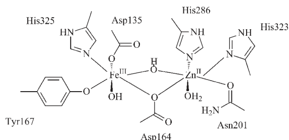
Figure 1. Representative active site of purple acid phosphatases (PAPs). The residue labels refer to red kidney bean PAP (rkbPAP).
