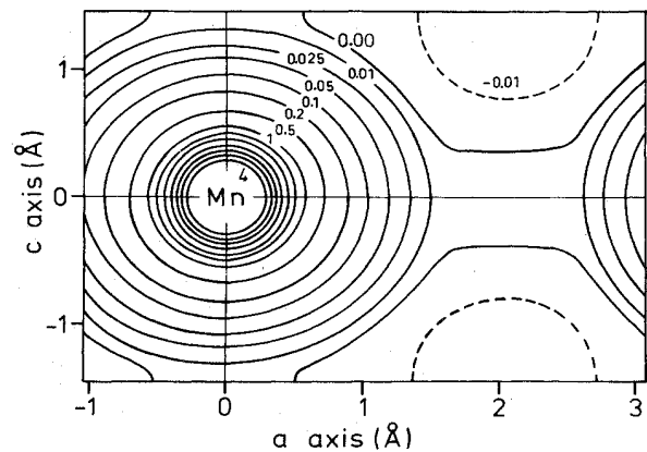
FIG. 12. Calculated spin-density distribution in the a - c plane. Units: electrons/ \text{\AA}^3 .
