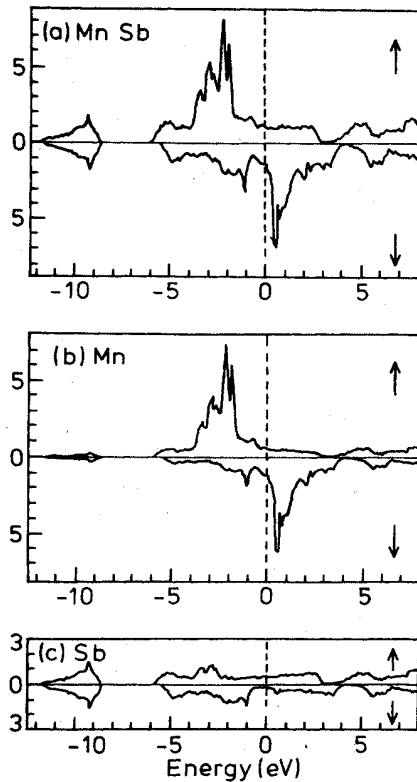
FIG. 5. (a) Total density of states of F-MnSb, (b) partial Mn density of states, (c) partial Sb density of states. Units: states \text{eV}^{-1}(\text{unit cell})^{-1} .
