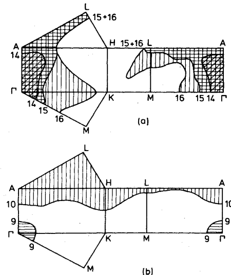
FIG. 15. Cross-sections of the Fermi surface with the boundary planes of the irreducible part of the Brillouin zone. Hole areas are shaded. (a) Majority-spin electrons. (b) Minority-spin electrons. The bands have been numbered in increasing energy order, starting with the Sb 5 s band.
