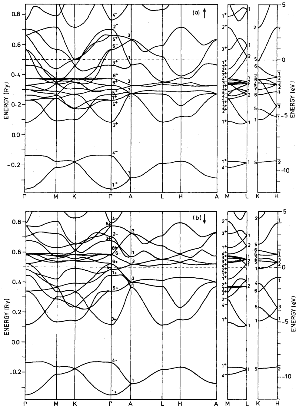
FIG. 4. Energy band structure of MnSb for (a) majority-spin and (b) minority-spin electrons. Ferromagnetic spin alignment.
