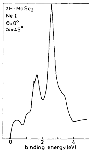
FIG. 9. Ne I ARUPS spectrum of \text{MoSe}_2 with \alpha=45^\circ at \theta=0^\circ .
