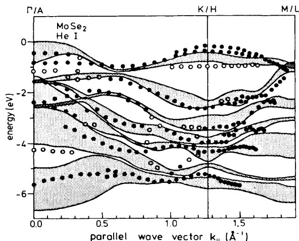
FIG. 11. Comparison of experimental and theoretical band structure of \text{MoSe}_2 . \Gamma K H A emission plane. He I radiation.
