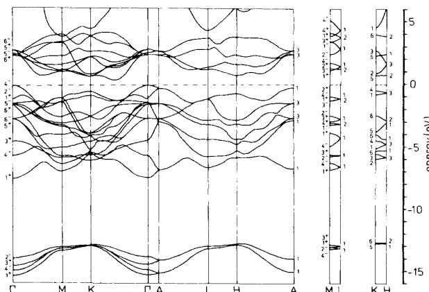
FIG. 4. Scalar relativistic band structure of 2H-WSe 2 .
