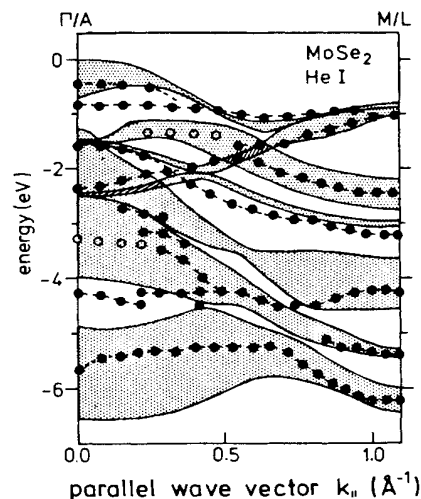
FIG. 10. Comparison of experimental and theoretical band structure of \text{MoSe}_2 . \Gamma M L A emission plane. He I radiation.
