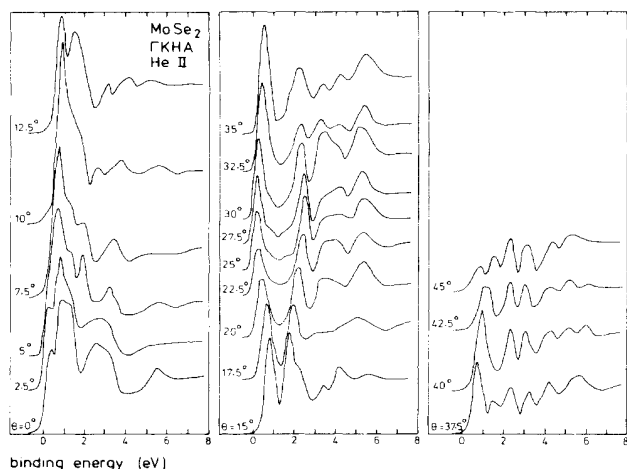
FIG. 8. He II ARUPS spectra of \text{MoSe}_2 with \alpha=45^\circ at different angles \theta in the \Gamma K H A plane.
