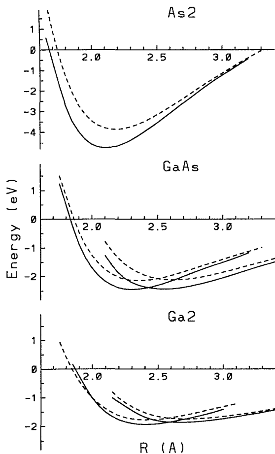
FIG. 1. Potential energy curves of diatomic molecules (a) \text{As}_2 ( ^1\Sigma_g^- ), (b) \text{GaAs} ( ^3\Sigma^- to the left and ^3\Pi to the right), and (c) \text{Ga}_2 ( ^3\Sigma^- to the left and ^3\Pi to the right). The result of the basis set DNP is plotted in solid lines and the result of the basis set dn is plotted in dashed lines. See the text for details.
