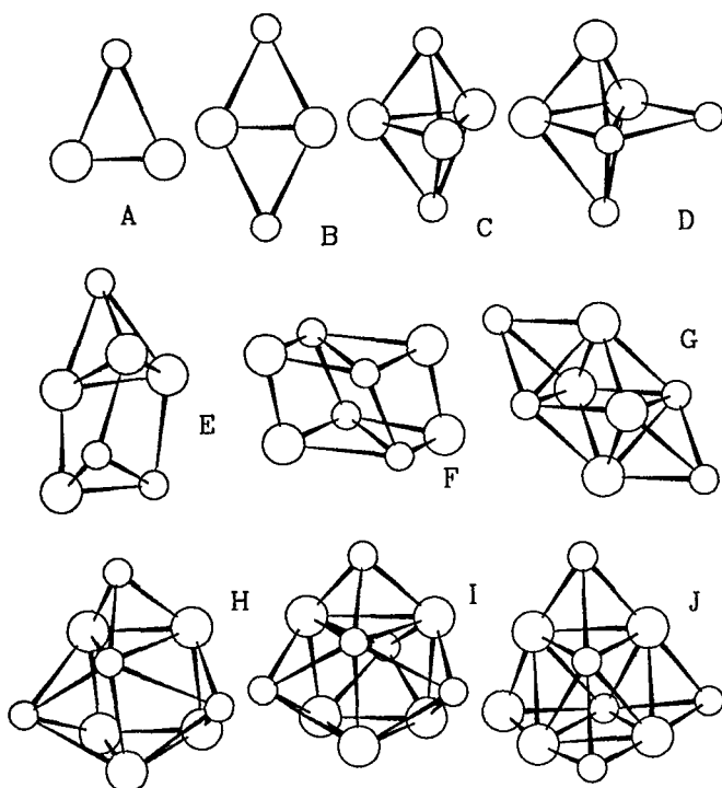
FIG. 2. Geometry of the most stable Ga_x As_y isomers with near x = y composition. The bigger circles represent As atoms and the smaller circles represent Ga atoms. Sticks are added between the balls intended to help for a three-dimensional perception, which do not necessarily represent a bond of any sort. The detailed geometries will be provided upon request. (a) GaAs_2 , isosceles triangle; (b) Ga_2As_2 , planar rhombus; (c) Ga_2As_3 , trigonal bipyramid; (d) Ga_3As_3 , edge capped trigonal prism; (e) Ga_3As_4 , capped trigonal prism; (f) Ga_4As_4 , rhombic prism; (g) Ga_4As_4 , bicapped octahedron; (h) Ga_4As_5 , TTP; (i) Ga_5As_5 , tetracapped trigonal prism (TTP); (j) Ga_5As_5 , tetracapped octahedron (TO).
