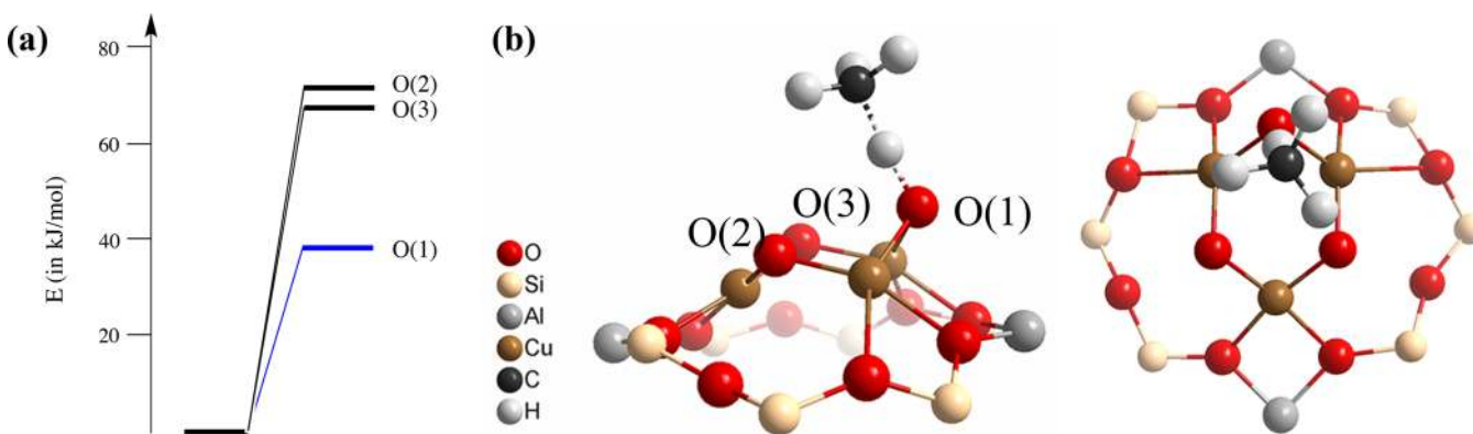
Figure 4. (a) Relative electronic energies of the C–H activation barriers (in kJ/mol, S = 1/2 ) from the three oxygen atoms of the [\text{Cu}_3(\mu\text{-O})_3]^{2+} cluster confined in MOR zeolite. (b) Optimized local geometry of the transition state of the C–H activation for O(1).
