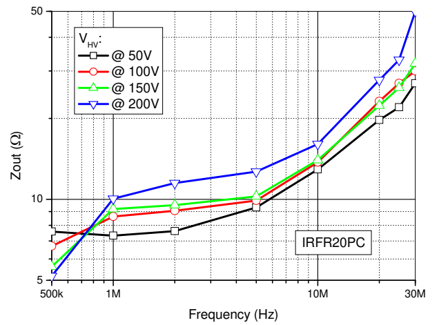
Fig. 8. Pulsar output impedance versus frequency.
