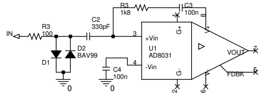
Fig. 12. Preamplifier input circuit topology with active input matching.
