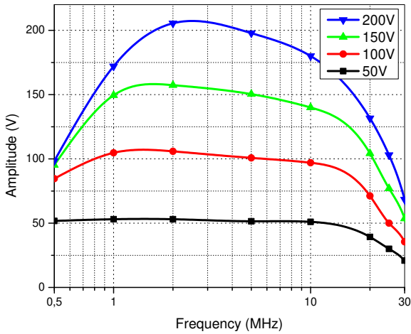
Fig. 7. Pulsar output AC response versus voltage swing \pm .
