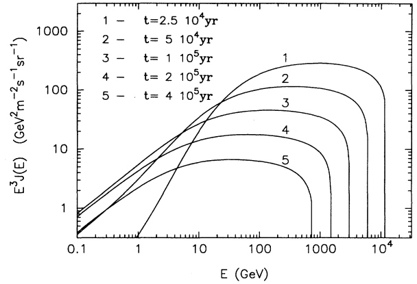
FIG. 1. The energy spectra of electrons at different times t after their injection into the ISM from a source at distance r = 100 pc. The calculated spectra correspond to a total energy output E_{\text{tot}} = 10^{48} erg in power-law primary electrons, \alpha = 2.2 , extending up to \gamma_{\text{max}} = 10^9 ; parameters of the diffusion coefficient are \delta = 0.6 , D_{10} \equiv D(10 \text{ GeV}) = 10^{28} \text{ cm}^2/\text{s} , and E_* = m_e c^2 \gamma_* = 3 \text{ GeV} ; a total energy output E_{\text{tot}} = 10^{48} erg is assumed.
