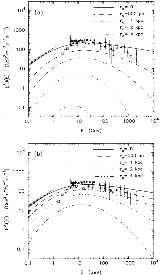
FIG. 2. The fluxes of electrons from sources continuously and uniformly distributed in the galactic disk, calculated for parameters \alpha = 2.4 , \delta = 0.6 , E_* = 3 GeV, and two different absolute values of the diffusion coefficient corresponding to (a) D_{10} = 10^{28} cm 2 /s, and (b) D_{10} = 10^{29} cm 2 /s. The total spectra (solid lines) are decomposed to show the spectral fluxes (contributions) coming from the sources at distances r \geq r_0 . The experimental fluxes correspond to the measurements by Taira et al. [11] (shown by solid triangles), Tang [19] (solid squares), Golden et al. [20] (open triangles), and Basini et al. [21] (open squares). The dashed region corresponds to the fluxes of CR electrons deduced from radio observations by Webber et al. [22].
