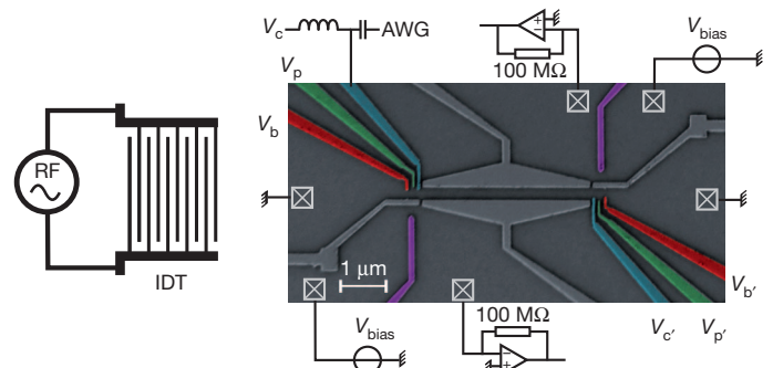
Figure 1 | Experimental device and measurement setup. Scanning electron microscope image of the single-electron transfer device, and diagram of the experimental setup. Two quantum dots, which can be brought into the single-electron regime, are separated by a 1D channel 3 \mu\text{m} long, as shown. Each quantum dot is capacitively coupled to a QPC close by that is used as an electrometer 9 . By applying a microwave burst 65 ns long on the IDT (see Methods for details), a train of about 150 moving quantum dots is created in the 1D channel. Gate V_c is connected to a home-made bias tee to allow nanosecond manipulation of the dot potential. RF, radio frequency.
