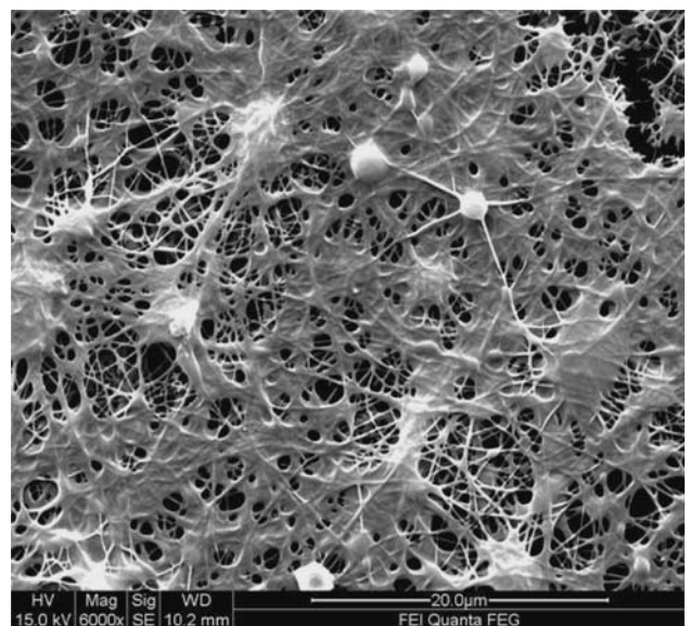
Fig. 4 SEM picture of PVA/aluminum nitrate nanofibers
