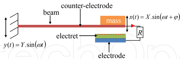
Figure 26. Cantilever-based electret energy harvesters [15]
