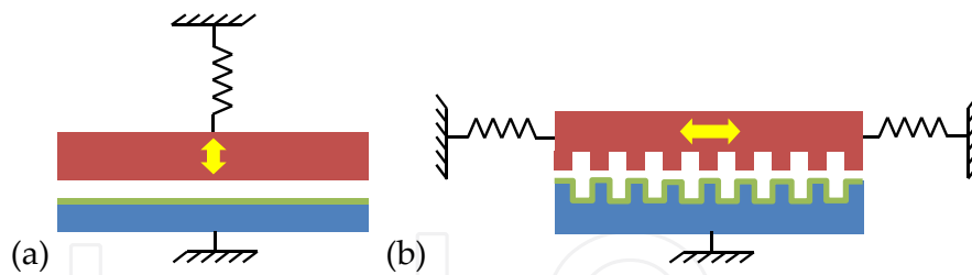
Figure 25. Standard architectures for electret-based Vibration Energy Harvesters
