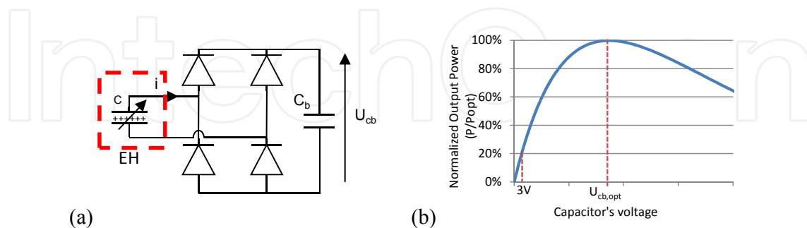
Figure 46. (a) Simple passive power converter – diode bridge-capacitor and (b) optimal output voltage on U_{cb}
