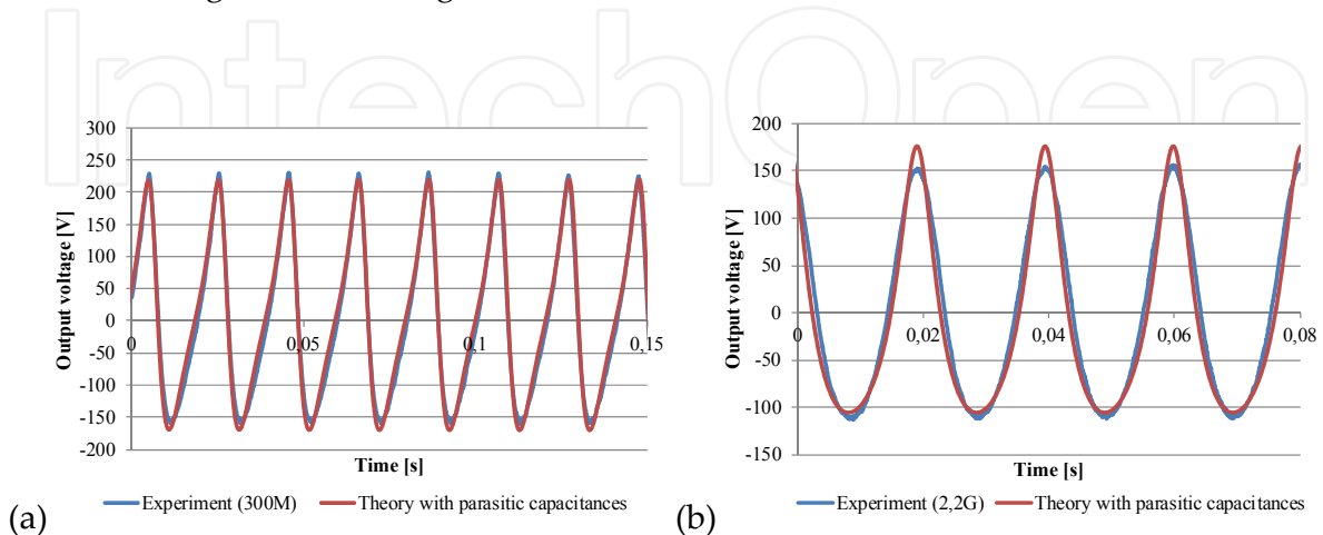
Figure 32. Validation of theory with a cantilever-based electret energy harvester (a) R=300MΩ and (b) R=2.2GΩ
