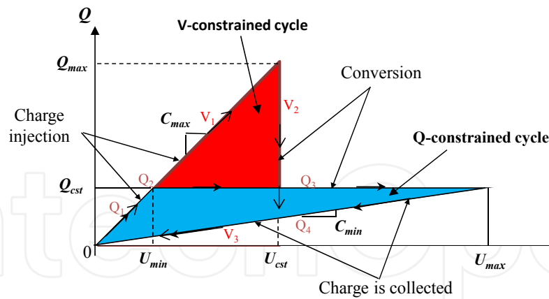
Figure 6. Standard energy conversion cycles for eletret-free electrostatic devices
