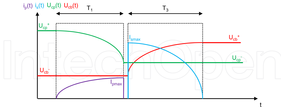
Figure 51. Voltages and currents during power conversion
