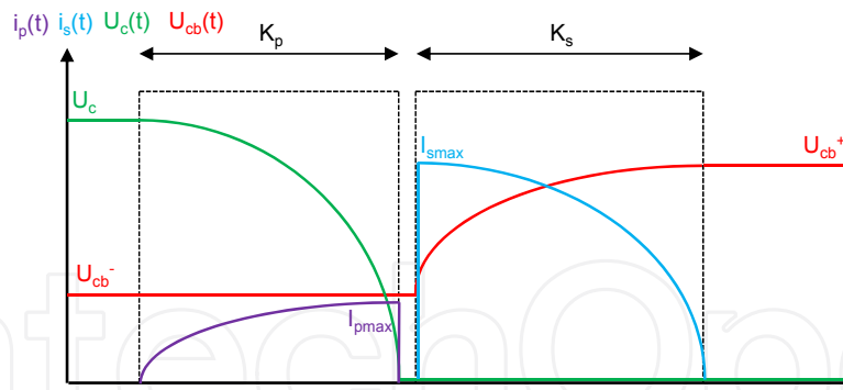
Figure 48. Voltages and currents during power conversion
