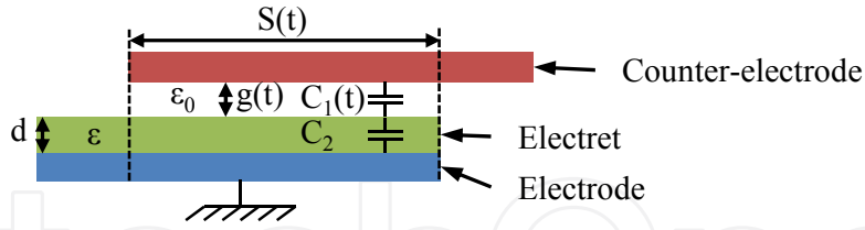
Figure 17. Capacitance of the simple plane capacitor
