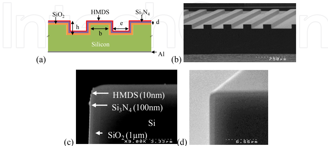
Figure 38. Patterned \text{SiO}_2/\text{Si}_3\text{N}_4 electrets from CEA-LETI [51]
