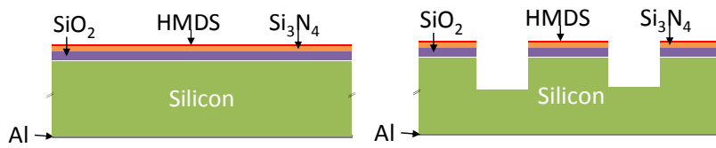
Figure 34. Obvious patterning that does not work
