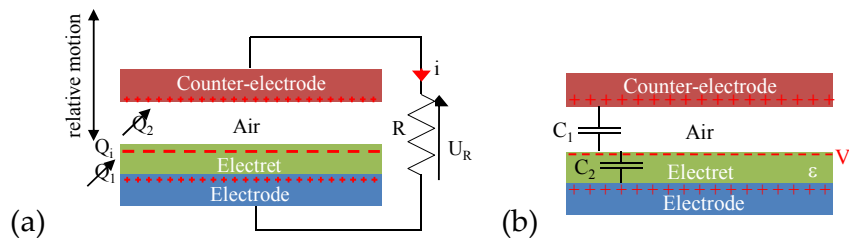
Figure 13. Electret-based electrostatic conversion – Concept
