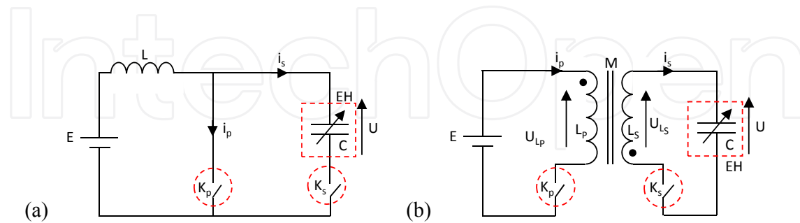
Figure 43. Bidirectional DC-to-DC converters (a) buck-boost and (b) flyback
