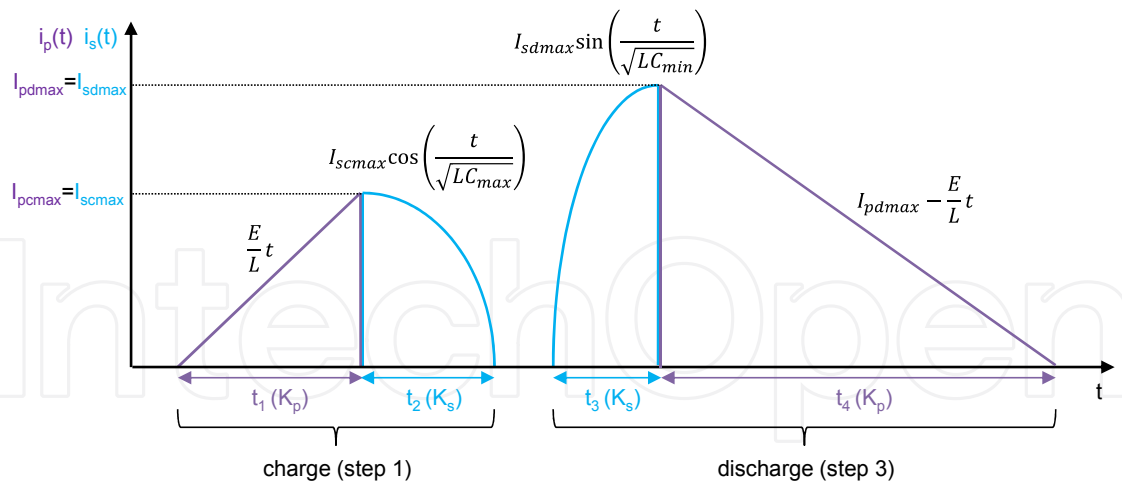
Figure 44. Waveforms of currents in buck–boost converters
