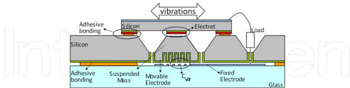
Figure 27. IMEC's first electret-based vibration energy harvester [32]
