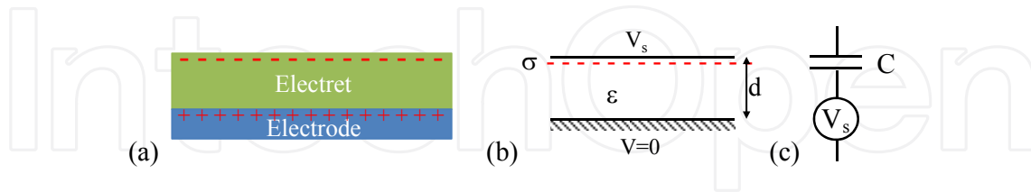
Figure 11. (a) electret layer (b) parameters and (c) equivalent model
