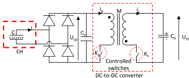
Figure 50. Energy transfer with pre-storage
