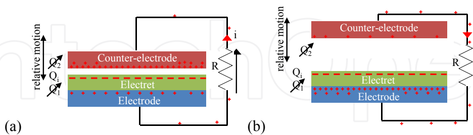
Figure 14. Electret-based electrostatic conversion – Charge circulation
