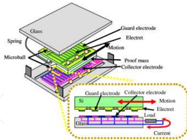
Figure 29. Device on microballs from [37]
