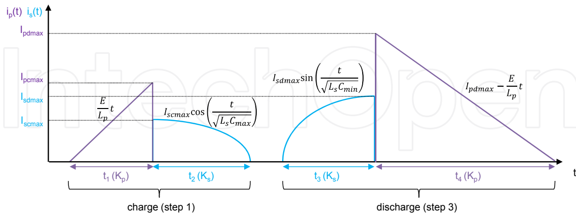
Figure 45. Waveforms of currents in flyback converters
