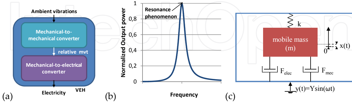
Figure 5. Vibration Energy Harvesters (a) concept (b) resonance phenomenon and (c) model
