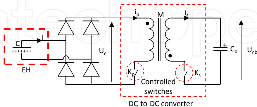
Figure 47. Energy transfer on maximum voltage detection
