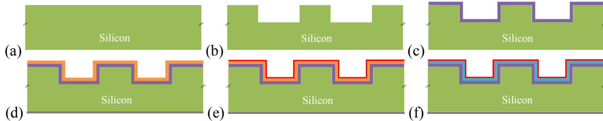
Figure 37. Fabrication process of CEA-LETI's DRIE-patterned electrets
