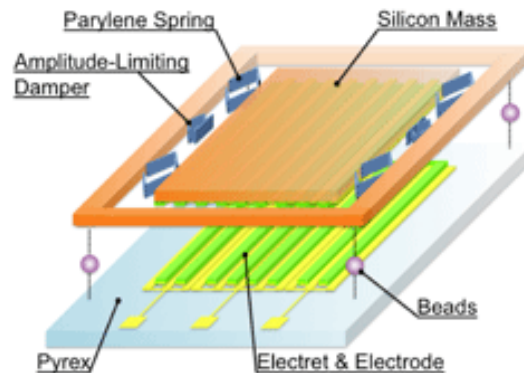
Figure 28. Multiphase electret energy harvester exploiting non-linear springs [38-39].
