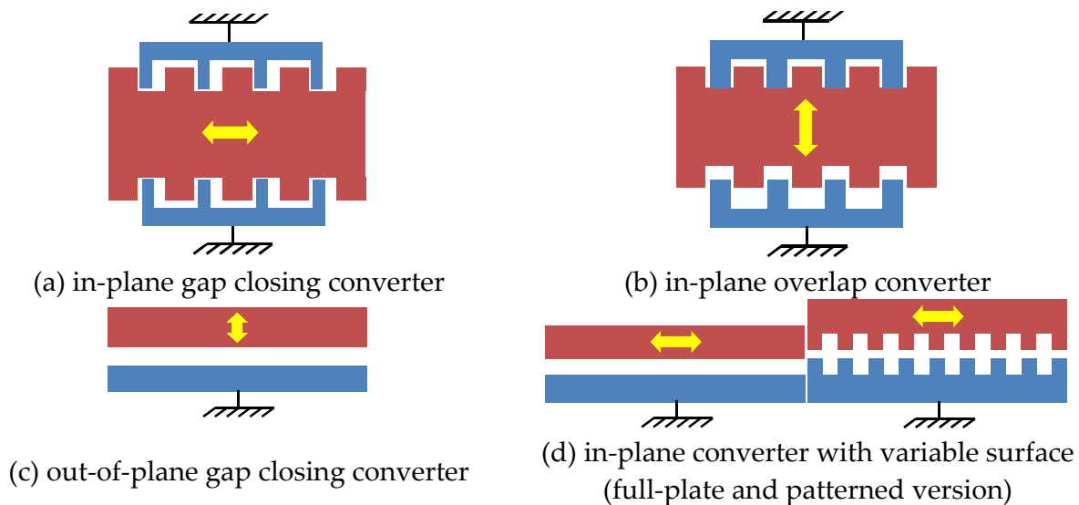
Figure 16. Basic capacitor shapes for electrostatic converters
