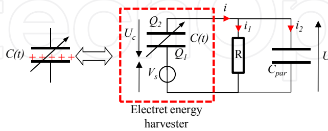
Figure 15. Electrical equivalent model of electret-based electrostatic converters
