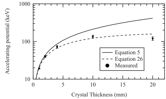
FIG. 7. Comparison of experimental data (Ref. 21) with the idealized model [Eq. (5a)] and with a model that accounts for charge leakage [Eq. (26)] for a one crystal system with a 5 \times 5 mm 2 rectangular LiTaO 3 crystal using \Delta T = 50 °C, R_g = 8 \times 10^{13} \Omega , \rho_{cr} = 10^{13} \Omega m, and dT/dt = 0.5 °C/s.
