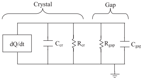
FIG. 6. Equivalent circuit showing the crystal and gap as lossy capacitors (Ref. 26).
