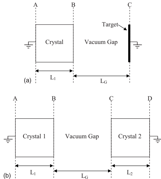
FIG. 1. (a) Sketch of a one-crystal system. (b) Sketch of a two-crystal system.
