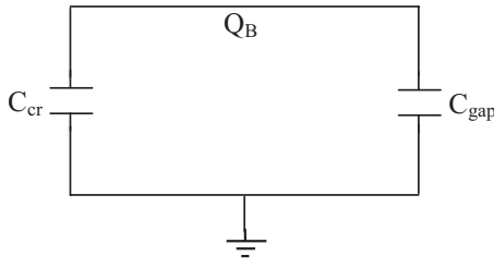
FIG. 2. The circuit diagram for the one-crystal system.
