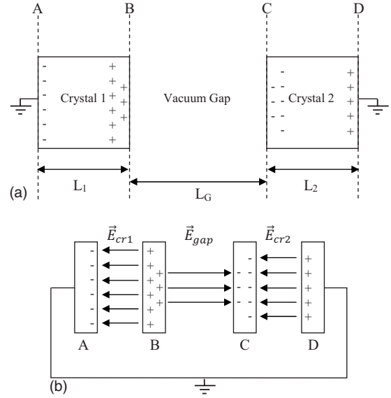
FIG. 5. (a) Sketch of a two-crystal system. The regions containing the charges near planes B and C are substantially magnified. (b) Sketch of the equivalent capacitors of (a) showing a magnified view of the surfaces located on planes A, B, C, and D. Not to scale.
