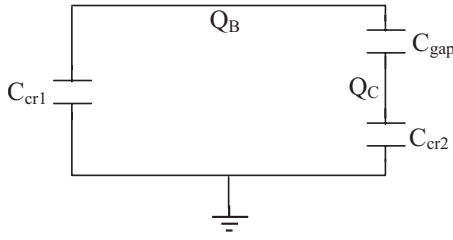
FIG. 4. A circuit diagram for the two-crystal system.
