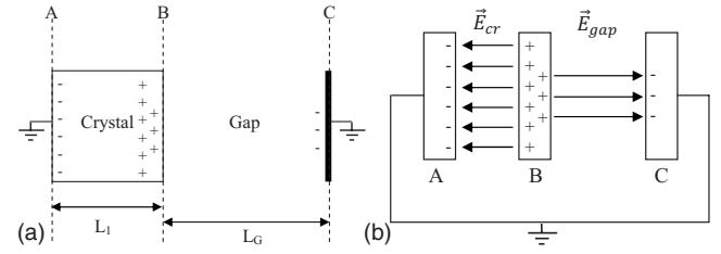
FIG. 3. (a) Sketch of the one-crystal system with example charges shown. The region containing the charges near plane B is substantially magnified. (b) Sketch of the equivalent capacitors of (a) showing a magnified view of the surfaces located on planes A, B, and C. Not to scale.
