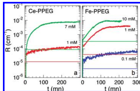
Figure 6. Same as Figure 4, but for PPEG–CeO 2 (a) and PPEG– \gamma -Fe 2 O 3 (b) nanoparticles.
