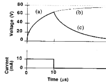
Fig. 3. Voltage on the 12- \text{mm}^2 area active center with respect to the outer ring of a coaxial electrode stimulated with 10- \mu\text{s} constant current pulses. (a) Charging region; (b) resistive heating region; (c) discharge region. Adapted from [105].
