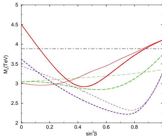
Figure 2: Lower bounds on M_c corresponding to the case \varepsilon^{H_1} = 1, \varepsilon^{H_2} = 0, \varepsilon^{q_L} = \varepsilon^{\ell_L} = \varepsilon^{u_R} = 1 (solid), \varepsilon^{H_1} = 1, \varepsilon^{H_2} = 0, \varepsilon^{q_L} = \varepsilon^{u_R} = \varepsilon^{e_R} = 1 (short-dashed), \varepsilon^{H_1} = 0, \varepsilon^{H_2} = 1, \varepsilon^{q_L} = \varepsilon^{\ell_L} = \varepsilon^{d_R} = \varepsilon^{e_R} = 1 (long-dashed) and \varepsilon^{H_1} = \varepsilon^{H_2} = 0, \varepsilon^{q_L} = \varepsilon^{\ell_L} = \varepsilon^{u_R} = \varepsilon^{d_R} = \varepsilon^{e_R} = 1 (dash-dotted). Thin (thick) lines correspond to SM (MSSM) 5D extensions.
