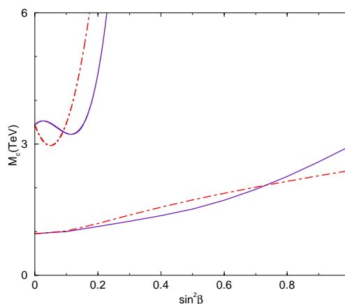
Figure 3: Lower (and upper) 95% c.l. bounds on M_c , as functions of s_\beta^2 , for the case \varepsilon^{H_2} = \varepsilon^{e_R} = \varepsilon^{d_R} = 1 , and \varepsilon^{H_1} = \varepsilon^{u_R} = \varepsilon^{\ell_L} = \varepsilon^{q_L} = 0 . Solid (dash-dotted) lines correspond to the MSSM (SM) case.
