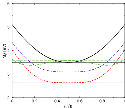
Figure 1: Lower bounds on M_c corresponding to the case \varepsilon^{H_1} = \varepsilon^{H_2} = 1 and \varepsilon^{\ell_L} = \varepsilon^{u_R} = \varepsilon^{d_R} = 1 (solid line), \varepsilon^{q_L} = \varepsilon^{e_R} = 1 (long-dashed), \varepsilon^{u_R} = \varepsilon^{d_R} = \varepsilon^{e_R} = 1 (short-dashed) and \varepsilon^{q_L} = \varepsilon^{\ell_L} = 1 (dash-dotted). Straight (non-straight) lines correspond to SM (MSSM) 5D extensions.
