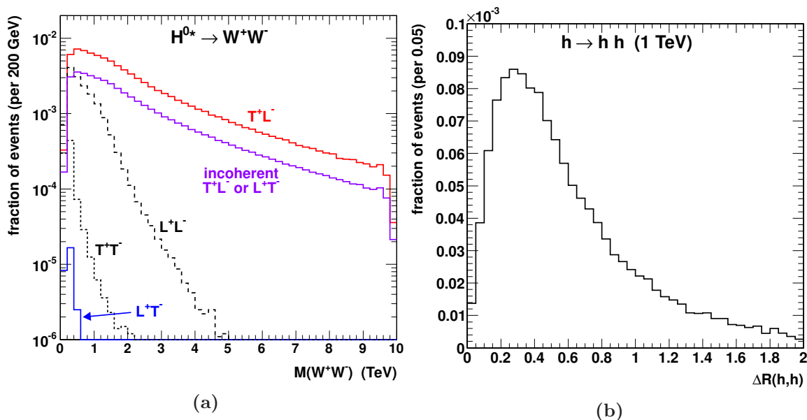
Figure 9. (a) W^+W^- invariant mass distributions from the EW splitting of a 10TeV h/Z_L ( H^{0*} ) \rightarrow W^+W^- , labeled by the helicities and charges as T^+L^- , L^+T^- , T^+T^- , and L^+L^- . The “incoherent T^+L^- or L^+T^- ” curve shows the corresponding result from showering h and Z_L states independently. (b) Kinematic \Delta R separation between the final state Higgs boson pair for the ultra-collinear splitting process h \rightarrow hh from a 1 TeV Higgs boson.
