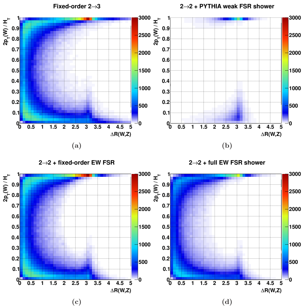
Figure 4. Event population for exclusive WZ + j production in the plane of 2p_T(W)/H_T versus \Delta R(W, Z) with p_T(j) \geq 3 TeV at a 100 TeV proton collider. (a) 2 \rightarrow 3 fixed-order WZj production generated with MadGraph; (b) 2 \rightarrow 2 dressed with the PYTHIA weak shower, which includes only q \rightarrow Vq splittings; (c) 2 \rightarrow 2 Wj and Zj production dressed with fixed-order FSR splitting functions; (d) 2 \rightarrow 2 dressed with the full EW FSR shower, including all collinear final-state Sudakov effects. QCD showering is not incorporated. An integrated luminosity of 10 \text{ ab}^{-1} is used for illustration.
