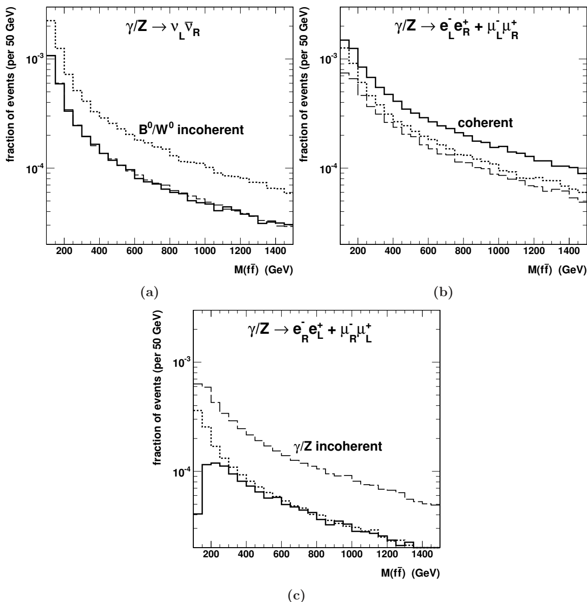
Figure 8. Invariant mass distributions for fermion pairs produced in the EW splitting of a 2.5 TeV \gamma/Z neutral boson, sourced by an e_L current, for exclusive final states (a) \nu_L \bar{\nu}_R , (b) \ell_L^- \ell_R^+ , and (c) \ell_R^- \ell_L^+ . Three treatments of the showering neutral bosons are: hypothetical incoherent B^0/W^0 (dotted), incoherent \gamma/Z (dashed), and the full coherent EW evolution (solid).
