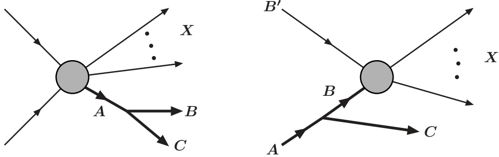
Figure 1. Schematic processes involving a collinear splitting A \rightarrow B + C in either the final state (left) or initial state (right).
