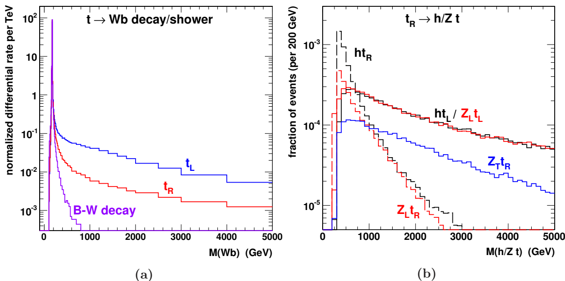
Figure 6. Invariant mass distributions for EW splittings initiated by a 10 TeV polarized top quark (a) for t_L \rightarrow Wb (top curve), t_R \rightarrow Wb (middle curve) and a fixed-width Breit-Wigner for unpolarized top decay without shower (lower curve); (b) for t_R \rightarrow ht_L/Z_L t_L , Z_T t_R (upper curves) and to ht_R , Z_L t_R (lower curves), respectively.
