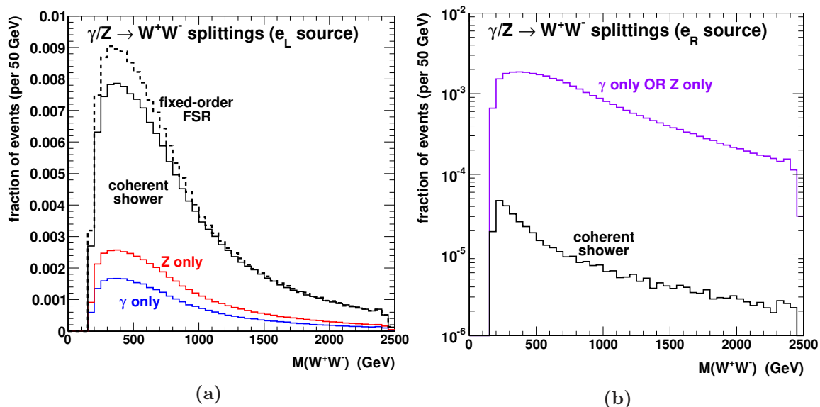
Figure 7. Invariant mass distributions for W^+W^- produced in the EW splitting of a 2.5 TeV \gamma/Z neutral boson, initiated from (a) e_L current with full coherent EW FSR (solid curve), fixed-order FSR (dashed curve), and the hypothetical incoherent \gamma or Z splittings (lower curves); (b) e_R current with full coherent EW FSR (solid curve) and the hypothetical incoherent \gamma or Z splittings (upper curve).
