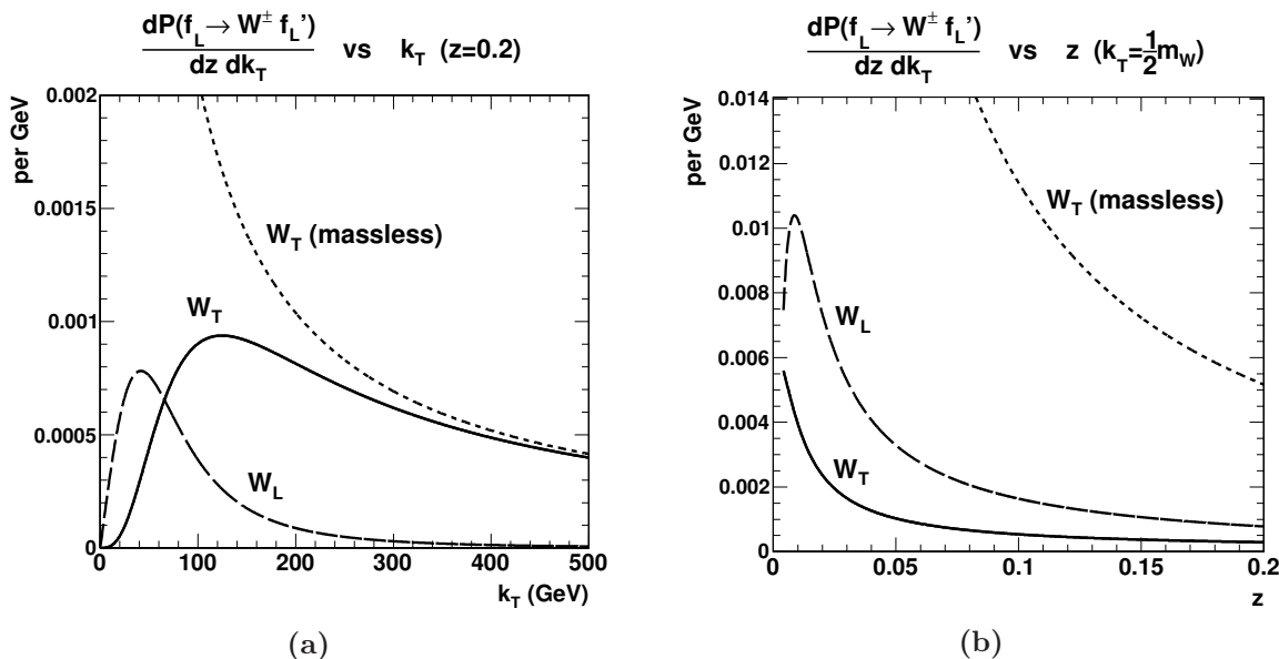
Figure 2. Fixed-order differential emission rate for W^\pm bosons off a massless fermion at E_f = 10 TeV: (a) k_T distribution at z = 0.2 , (b) z distribution at k_T = m_W/2 . The different curves correspond to massless transversely-polarized W_T^\pm (dotted curves), massive transversely-polarized W_T^\pm (solid curves), and massive longitudinally-polarized W_L^\pm (dashed curves).
