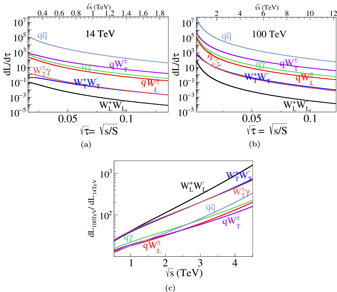
Figure 3. Representative parton luminosities in pp collisions at (a) \sqrt{S} = 14 TeV, (b) \sqrt{S} = 100 TeV, and (c) the ratio of luminosities between the two beam energies as a function of partonic CM energy \sqrt{s} .
