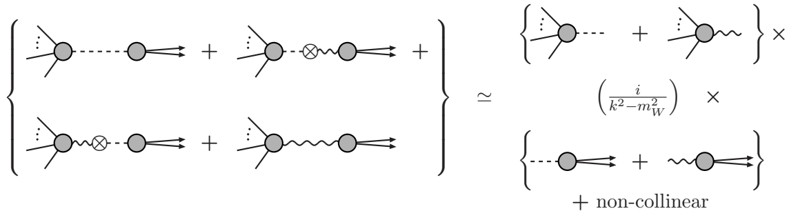
Figure 11. Schematic tree-level collinear factorization for an arbitrary process with a splitting Goldstone/longitudinal in the final state.
