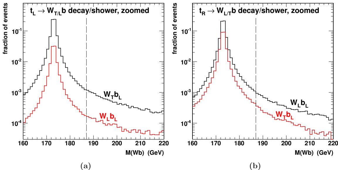
Figure 12. Invariant mass distributions for EW decay/showering of a 10 TeV polarized top quark for (a) conventional-collinear t_L \rightarrow W_T^+ b_L and ultra-collinear t_L \rightarrow W_L^+ b_L , and (b) conventional-collinear t_R \rightarrow W_L^+ b_L and ultra-collinear t_R \rightarrow W_T^+ b_L . Decay and shower are matched at 187 GeV (vertical dashed line). The conventional-collinear contributions correspond to the upper histograms, while the ultra-collinear contributions correspond to the lower histograms.
