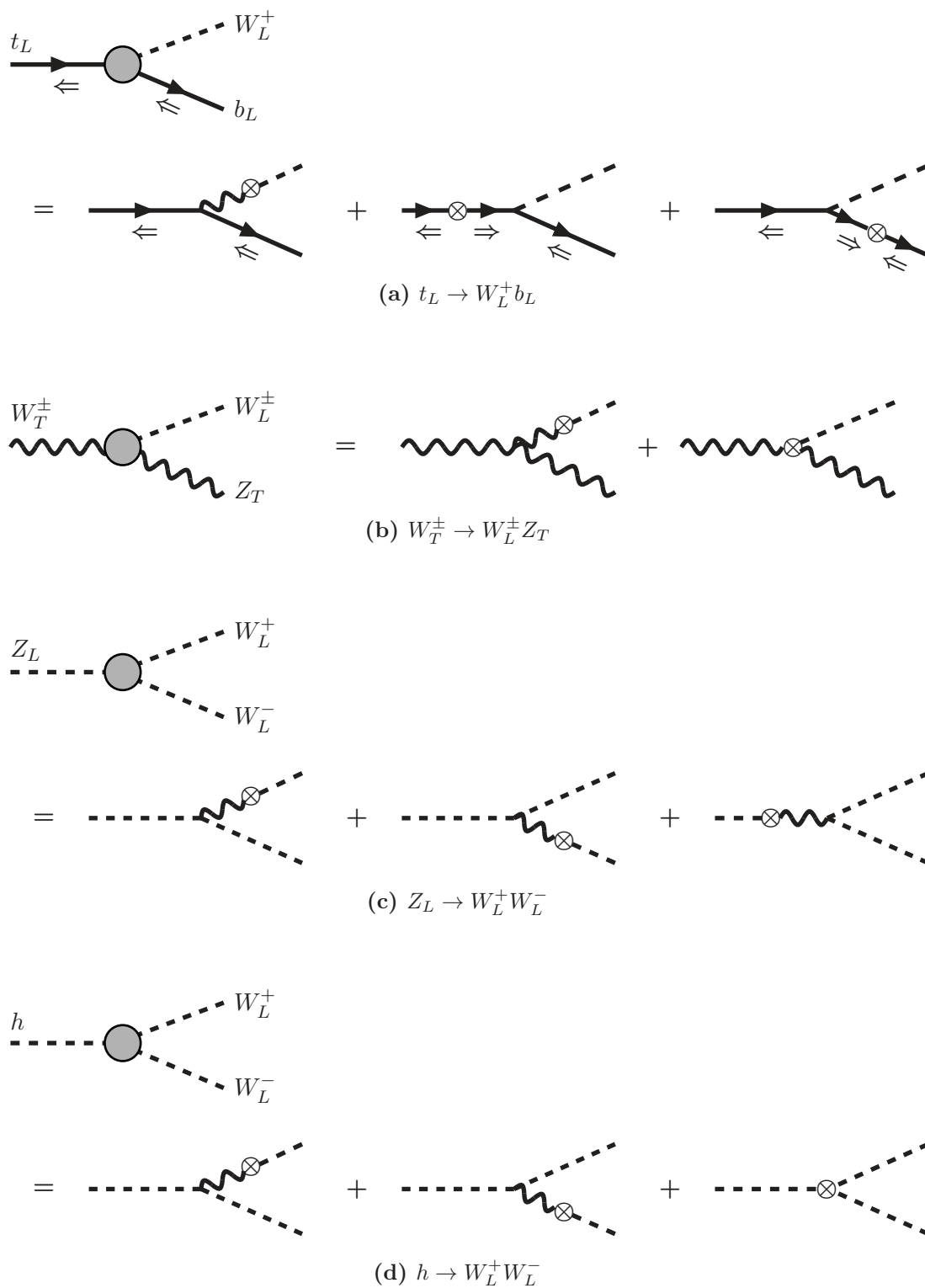
Figure 13. Representative ultra-collinear splittings with multiple contributing diagrams. The effects of the VEV are indicated schematically by the symbol \otimes .
