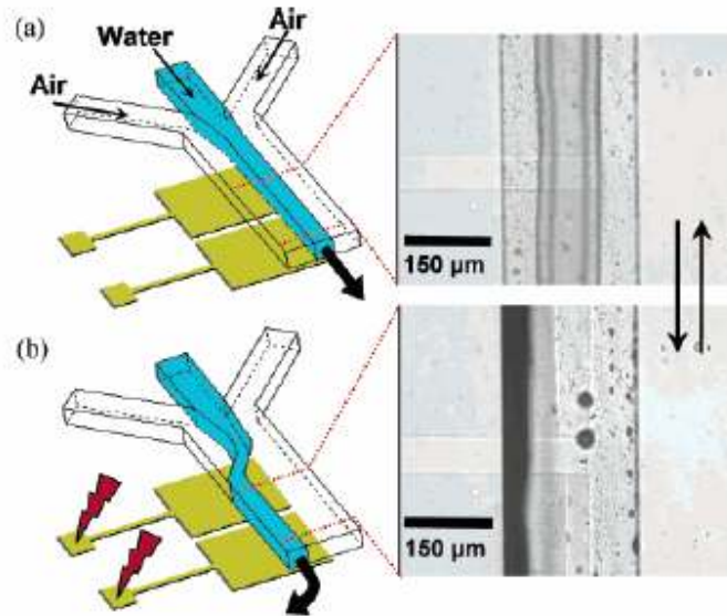
Figure 26. Electrically induced switching of surface energy caused (a) a focused high-speed water stream in the middle to (b) swerve to its right (relative to the direction of fluid flow), guiding the flow along the sidewall. Water was injected at 20 mL/h, and air flows were driven by 400 mmHg vacuum at the outlet. Channel height is 100 \mu\text{m} . (reproduced with permission from ref. [70])
