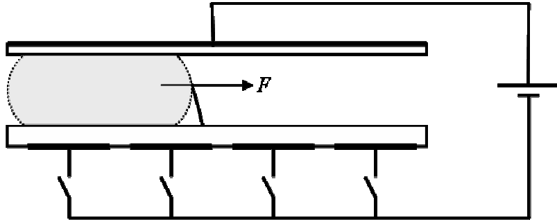
Figure 25. Schematic of a typical lab-on-a-chip system. The thin white layer on the top surface is usually a hydrophobic top coating that does not insulate the droplet electrically. By activating the second electrode, the bottom right contact angle is reduced and the droplet is distorted accordingly.
