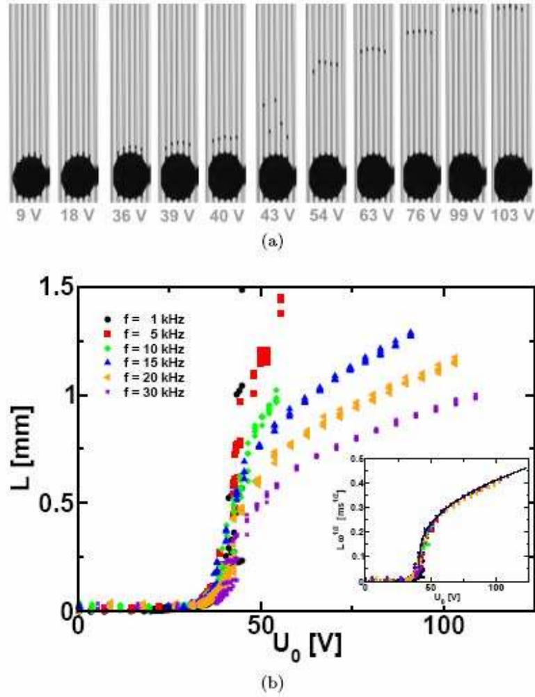
Figure 18. (a) Top-view of the channels for different voltages. The frequency of the voltage is 20 kHz and the drop wets 5 channels. On the right of the drop one see the contacting electrode. (b) Measurements of the length as a function of the applied voltage for different frequencies. The threshold voltage is obtained at 43 V. Inset: rescaled data. (courtesy of R. Seemann and J.-C. Baret)
