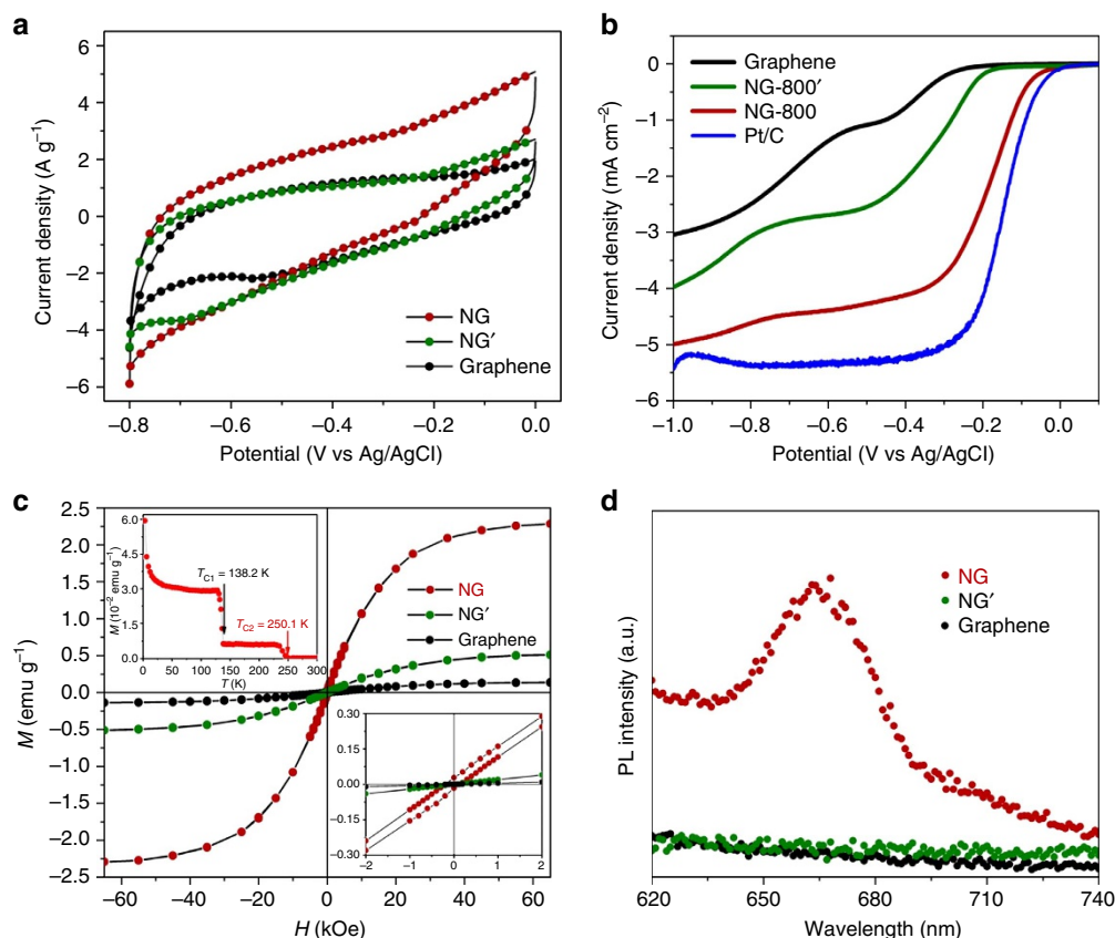
Figure 5 | Performance of superdoped graphene with a high level of N. (a) Representative CV curves of graphene, NG' and NG in 6 M KOH solution at a scan rate of 5 \text{ mVs}^{-1} . (b) Linear sweep voltammetry (LSV) curves for graphene, NG-800', NG-800 and Pt/C on a rotating disk electrode (RDE; 1,600 r.p.m.) in 0.1 M KOH solution with a scan rate of 5 \text{ mVs}^{-1} . (c) Typical M-H curves of graphene, NG' and NG measured at 2 K. Insets are the M-T curve of NG measured from 2 to 300 K under an applied field H = 500 \text{ Oe} (top left of panel) and part of the magnetization curves (bottom right of panel). (d) PL spectra of graphene, NG' and NG excited at 500 nm.
