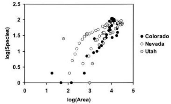
Fig. 2. Species-area curves for each state. Shown are the log transformed numbers of species and number of km 2 in each elevational band in each state.
