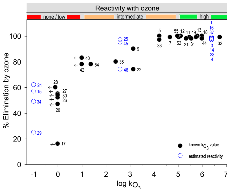
Figure 1 Elimination of micropollutants during ozonation of hospital wastewater (1.08 \text{gO}_3/\text{gDOC} , 7 \text{mg/L O}_3 , pH 8.5) versus ozonation rate constants from literature ( \text{M}^{-1}\text{s}^{-1} , Table S11) or estimated reactivity at pH 8-8.5 (Table S6) if k_{\text{O}_3} is not available. Arrows represent \log k_{\text{O}_3} < 1 or 10, respectively. See Table 1 for micropollutant numbering. Micropollutants for which quantification of elimination was limited by LOQ (2, 6, 8, 10, 19, 35, 38, 39, 41, 43, 47, 48, 50, 51, 53, and 56) are not included.
