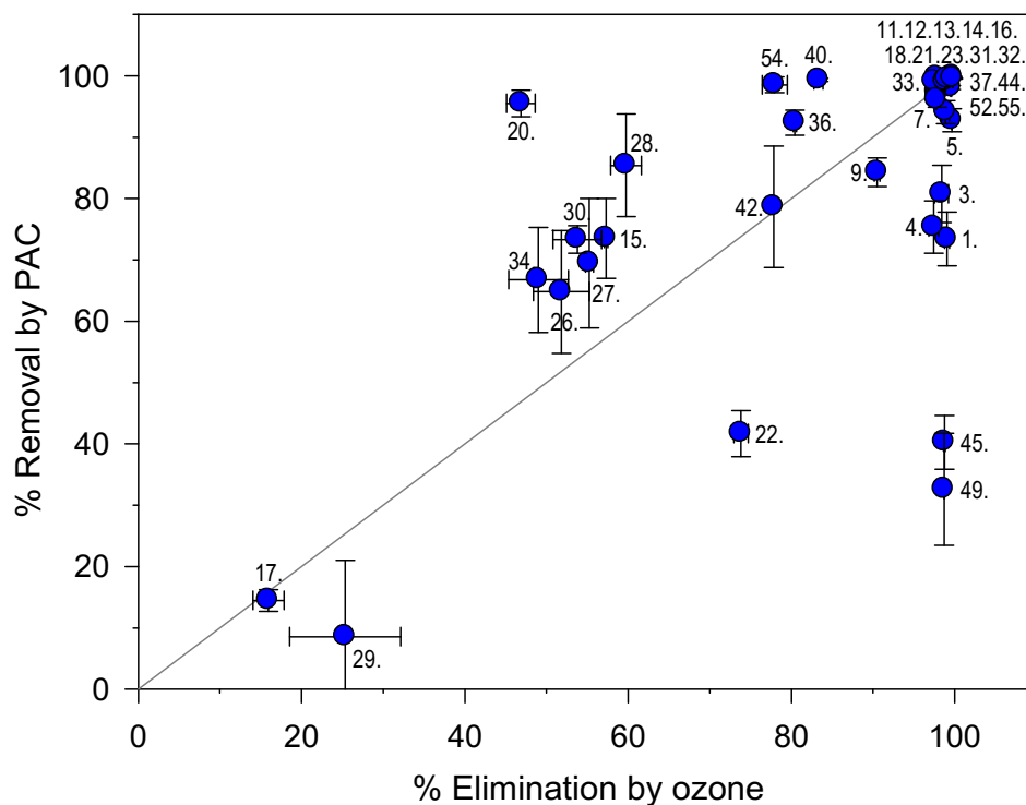
Figure 3. Comparison of micropollutants' elimination by ozone and PAC. Ozone dose: 7 \text{ mg/L} ( 1.08 \text{ gO}_3/\text{gDOC} , \text{pH } 8.5 ); PAC dose: 23 \pm 7 \text{ mg/L} , \text{pH } 8.8 . See Table 1 for micropollutant numbering.
