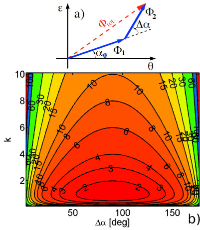
Fig. 1. (a) MO contributions \Phi_1 , \Phi_2 to the total MO effect \Phi_{tot} displayed in \theta, \epsilon plane. (b) Dependence of condition number \kappa(\mathbf{A}) of 2 \times 2 matrix \mathbf{A} of two column vectors \Phi_1 , \Phi_2 on angle \Delta\alpha between the vectors and parameter k corresponding to the ratio of absolute values |\Phi_1|, |\Phi_2| . See Eq. (5).
