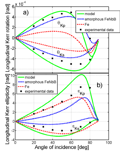
Fig. 3. Calculated dependence of longitudinal Kerr effect: (a) rotation, (b) ellipticity on angle of incidence for spherical Fe particles in homogeneous FeNbB material. The wavelength of incident light is 670 nm. The contributions from Fe and from FeNbB are also shown separately. The model is compared with experimental data from [9] (square dots).
