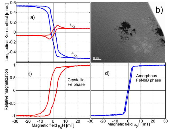
Fig. 2. (a) Sketch of the MO longitudinal Kerr rotation \theta_{Ks} and ellipticity \epsilon_{Ks} measured on wheel side of FeNbB ribbon for incident s -polarized wave at wavelength 670 nm and angle of incidence 65^\circ . (b) Transmission electron microscopy on wheel side of the FeNbB ribbon. Dark and light areas show the crystalline \alpha -Fe phase. (c), (d) Hysteresis loops of the crystalline Fe phase and the amorphous FeNbB phase separated from data in (a), respectively.
